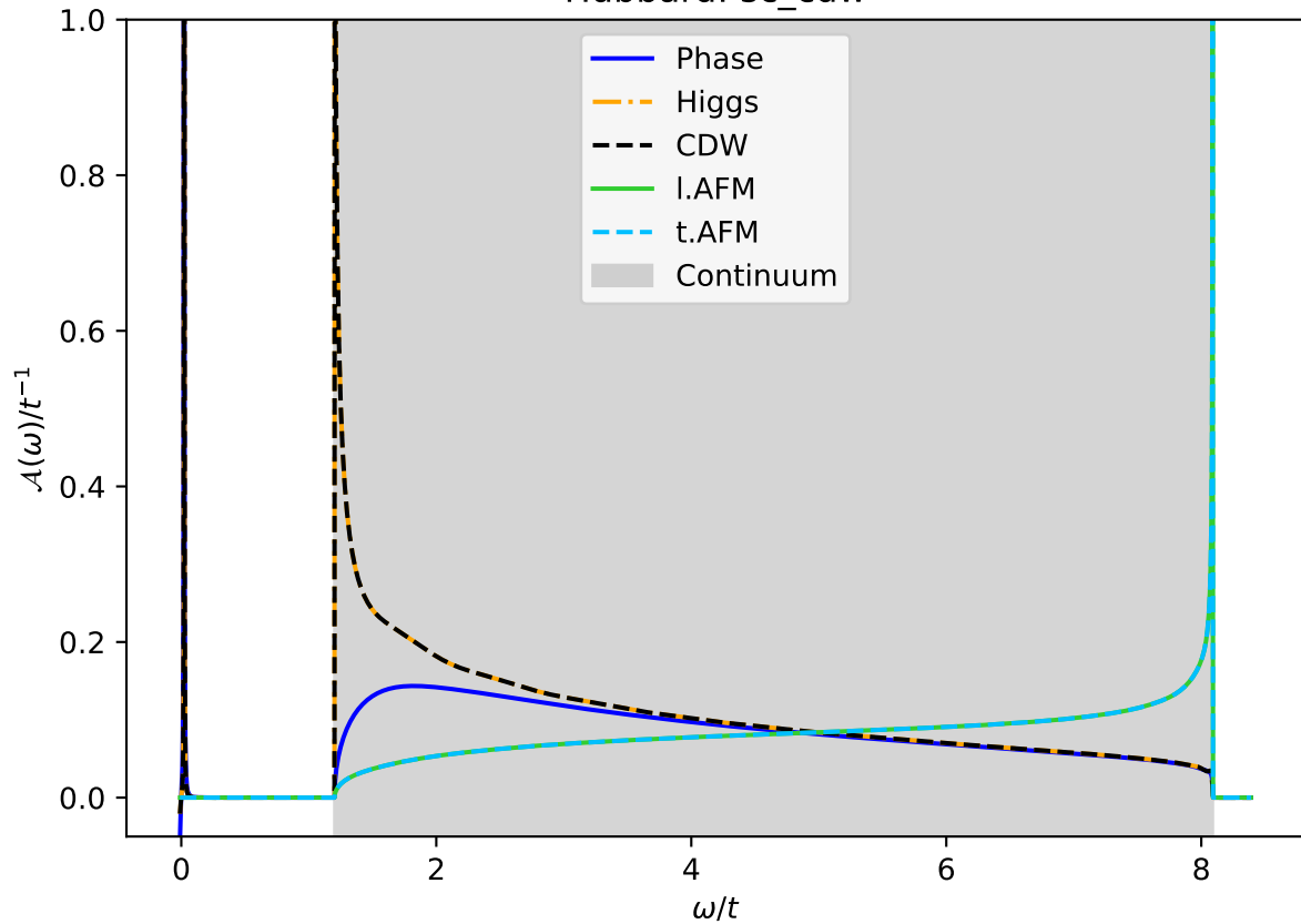
Hubbard: sc_cdw
