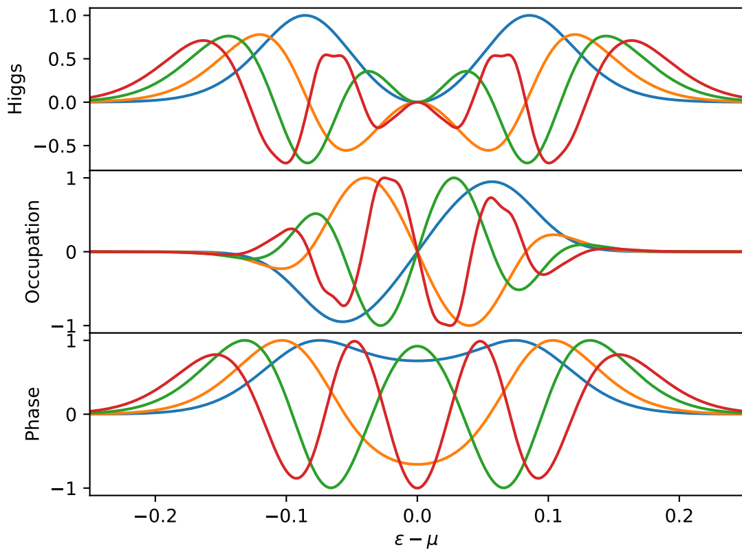
LatticeCUT: standard
