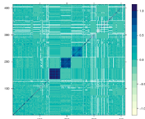
Kendall's \tau
