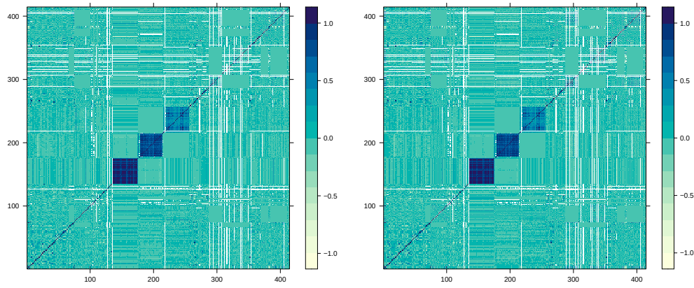
(a) Pearson's r
