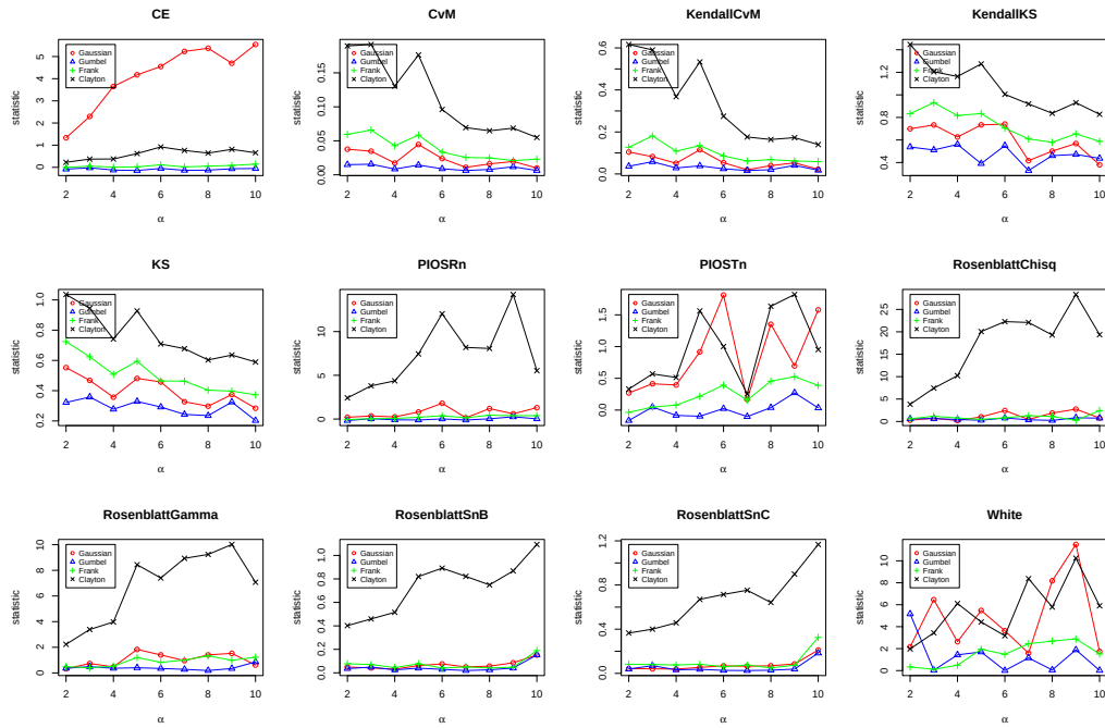
Figure 4.20: Results of the copula hypothesis tests in the simulation with Gumbel copula.
