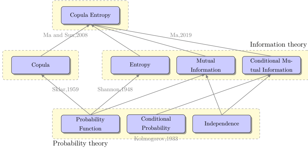
Figure 1.1: Relationships between the theories.
