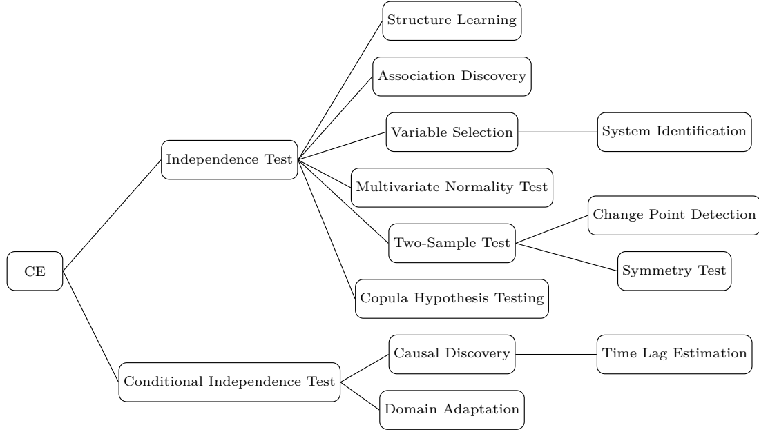
Figure 3.1: Relations between the theoretical applications of CE.
