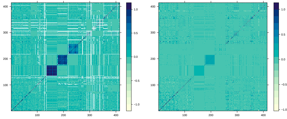
(c) Kendall's \tau
