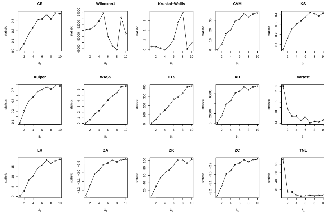
(b) Simulations based on changing variance
