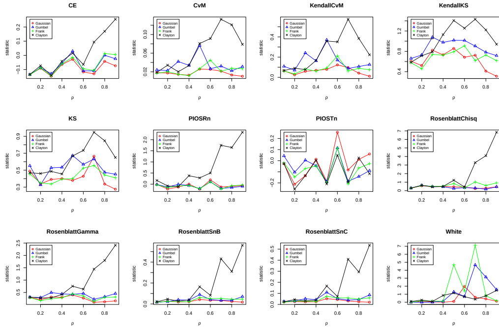
Figure 4.19: Results of the copula hypothesis tests in the simulation with Gaussian copula.
