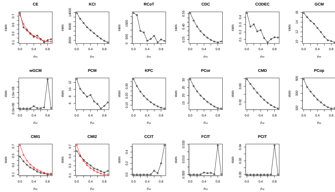
Figure 4.7: Results of simulation experiments on trivariate normal copulas (red line for true value).
