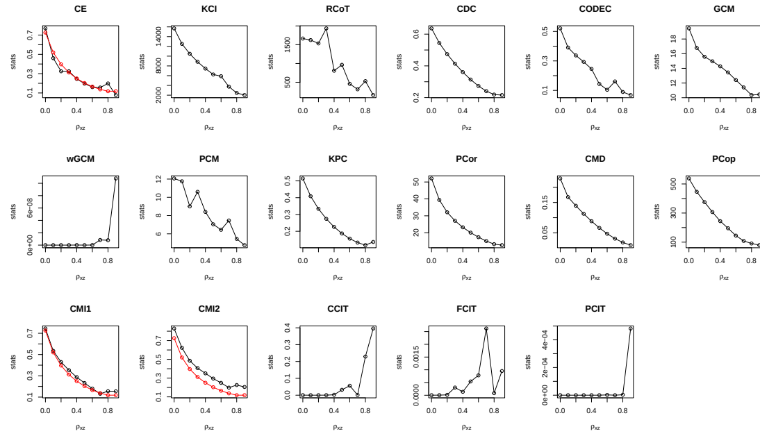
Figure 4.6: Results of simulation experiments on trivariate normal distributions (red line for true value).
