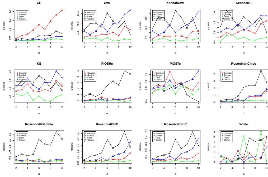
Figure 4.21: Results of the copula hypothesis tests in the simulation with Frank copula.
