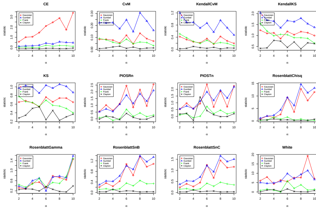
Figure 4.22: Results of the copula hypothesis tests in the simulation with Clayton copula.
