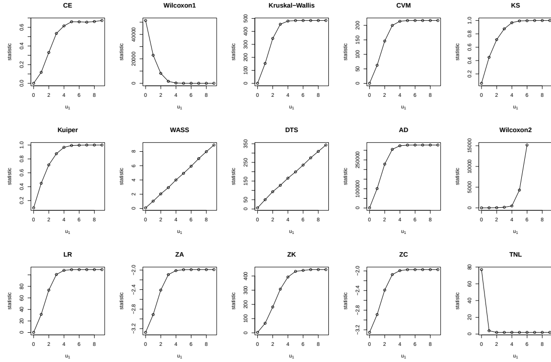
(a) Simulations based on changing mean
