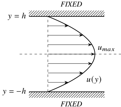
(b) POISEUILLE FLOW
