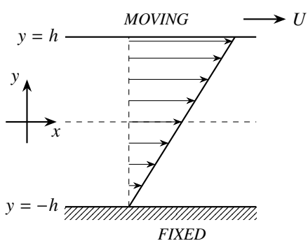
(a) COUETTE FLOW
