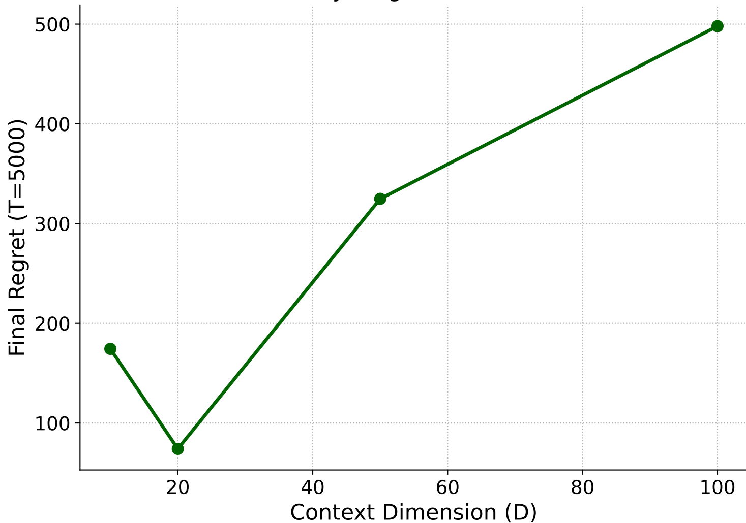
Scalability (Regret vs Dimension)
