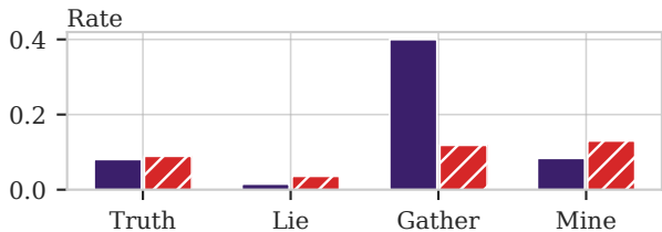
Cooperation Rate
