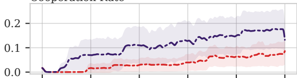
Cooperation Rate
