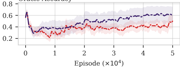
Oracle Accuracy
