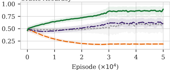
Oracle Accuracy
