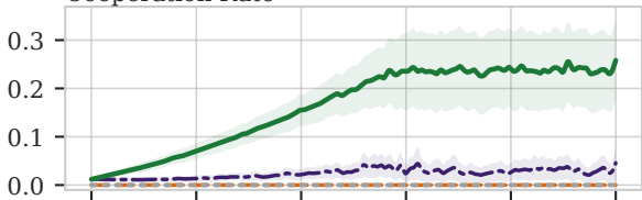
Cooperation Rate
