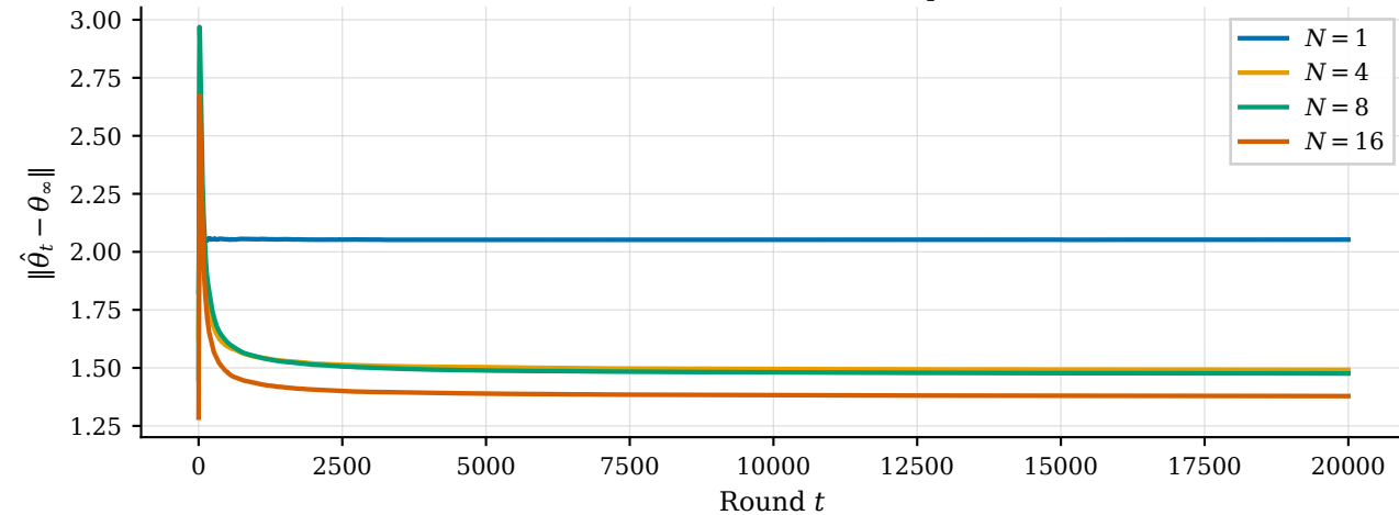
(b) Distance to biased fixed point
