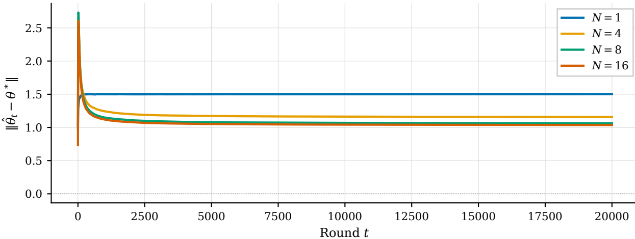
(a) Distance to truth
