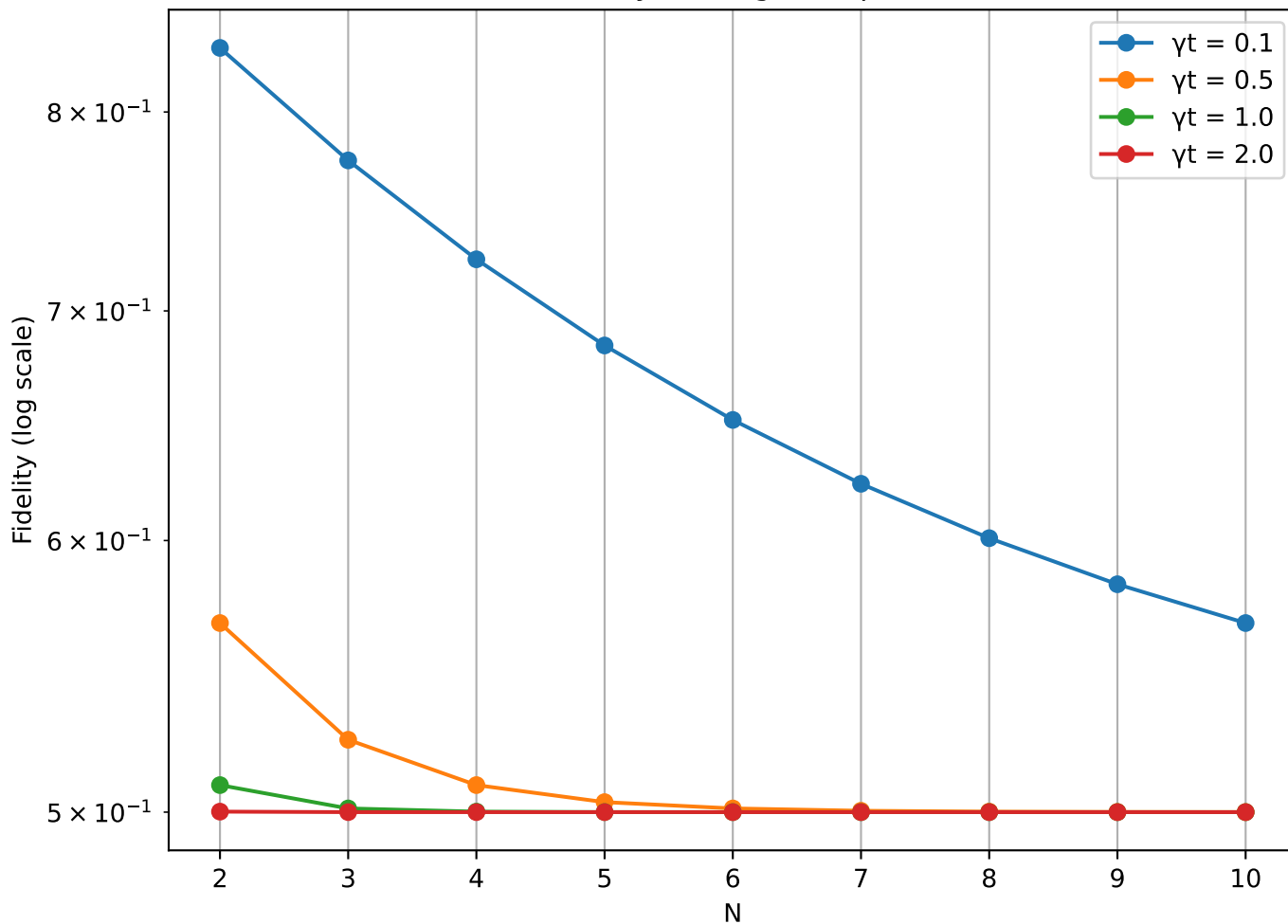
GHZ Fidelity Scaling (independent)
