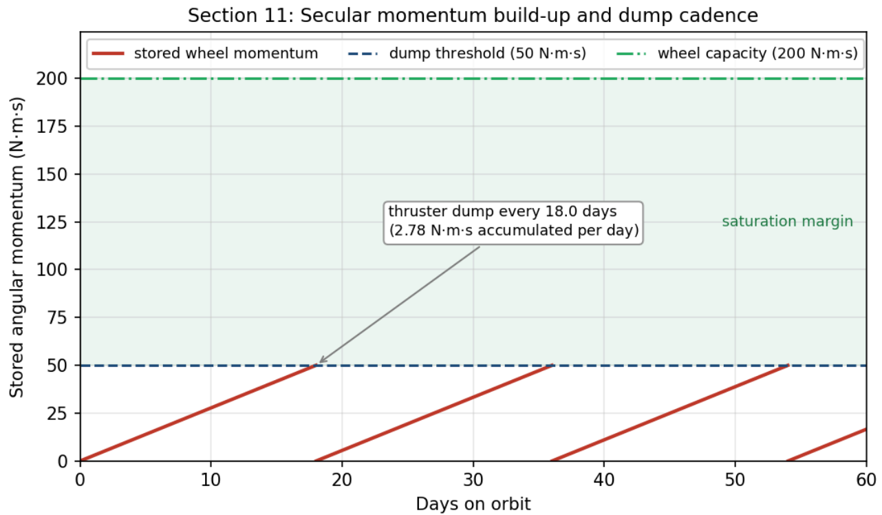
Figure 8: SRP torque at GEO is secular, so the wheels ramp and must be desaturated with thrusters, not magnetorquers.
