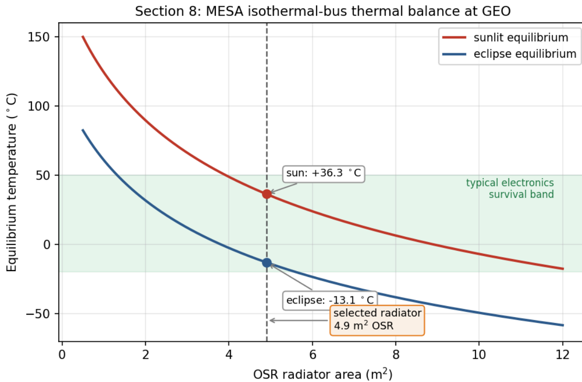
Figure 5: Sizing the radiator is a trade between the sunlit and eclipse cases; heaters close the remaining eclipse gap.
