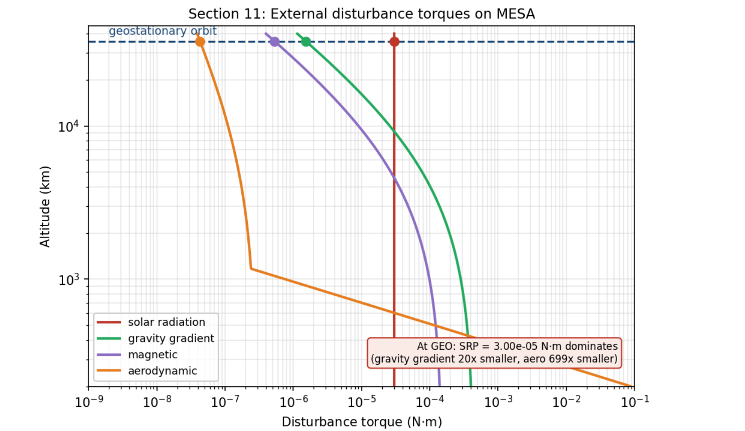
Figure 6: Torque magnitudes for the MESA geometry. Markers are the GEO operating point; SRP sets the ADACS design.
