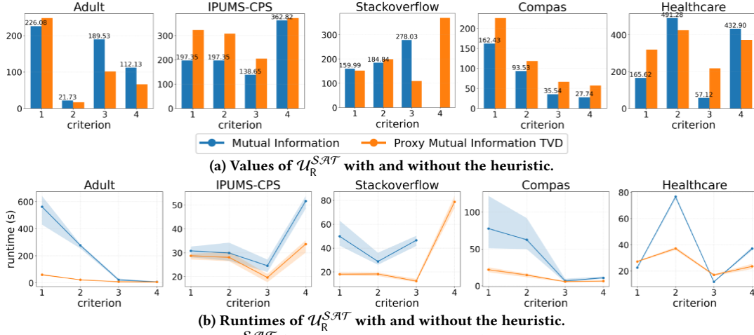
Figure 9: Comparison of \mathcal{U}_R^{SAT} (computed by Algorithm 2) with and without the heuristic.
