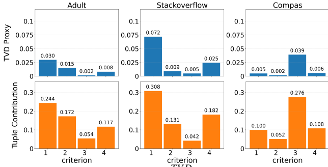
Figure 10: Comparison of \mathcal{U}_R^{TVD} and \mathcal{U}_R^{TC} without privacy considerations.
