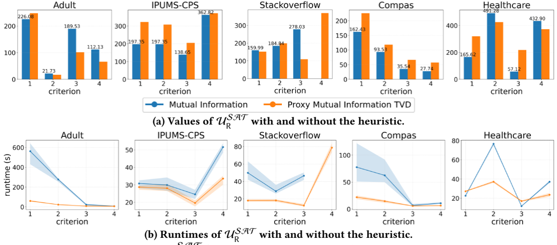
Figure 9: Comparison of \mathcal{U}_R^{\text{SAT}} (computed by Algorithm 2) with and without the heuristic.
