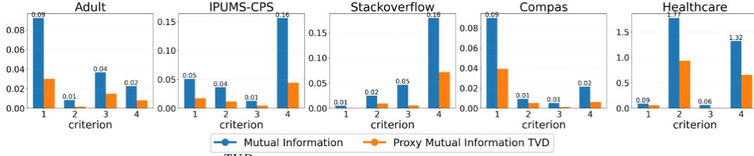
Figure 7: Faithfulness of noisy \mathcal{U}_{MI}^{TVD} to noisy \mathcal{U}_{MI} over different datasets and fairness criteria from Table 2.
