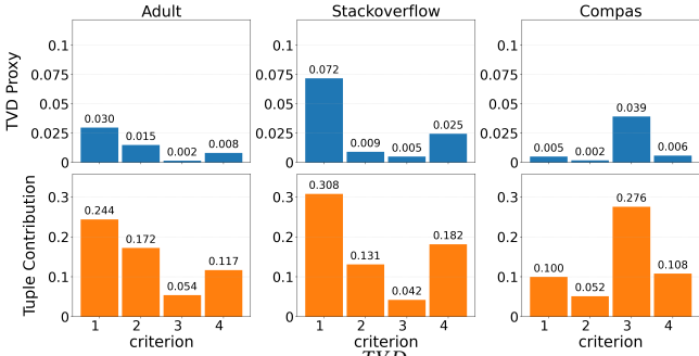
Figure 10: Comparison of \mathcal{U}_{\text{MI}}^{\text{TVD}} and \mathcal{U}_{\text{TC}} without privacy considerations.
