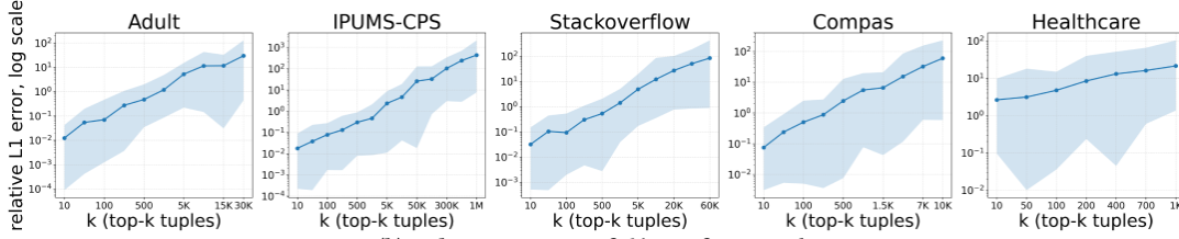
(b) Relative L1 error of \mathcal{U}_{TC} as function k .
