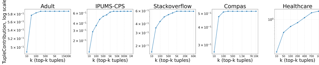
(a) Non-noisy value of \mathcal{U}_{TC} as function of k .
