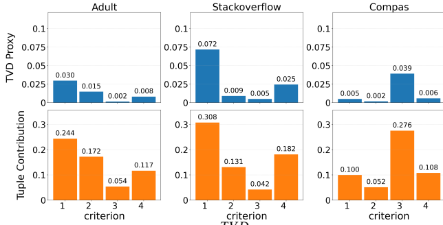
Figure 10: Comparison of \mathcal{U}_{MI}^{TVD} and \mathcal{U}_{TC} without privacy considerations.
