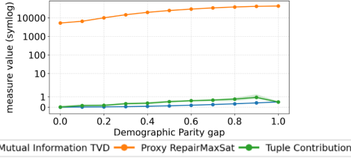
Figure 4: Change of measure values as the Demographic Parity in the dataset gradually increases.
