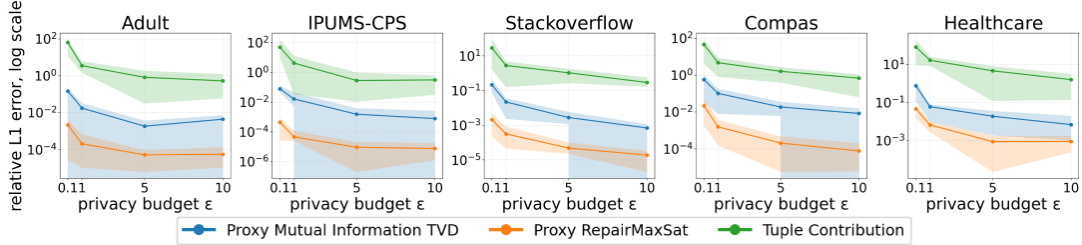
Figure 6: Relative L1 error as function of privacy budget for the datasets and criteria from Table 2.
