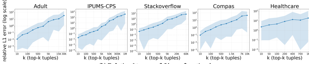
(b) Relative L1 error of \mathcal{U}_{TC} as function k .
