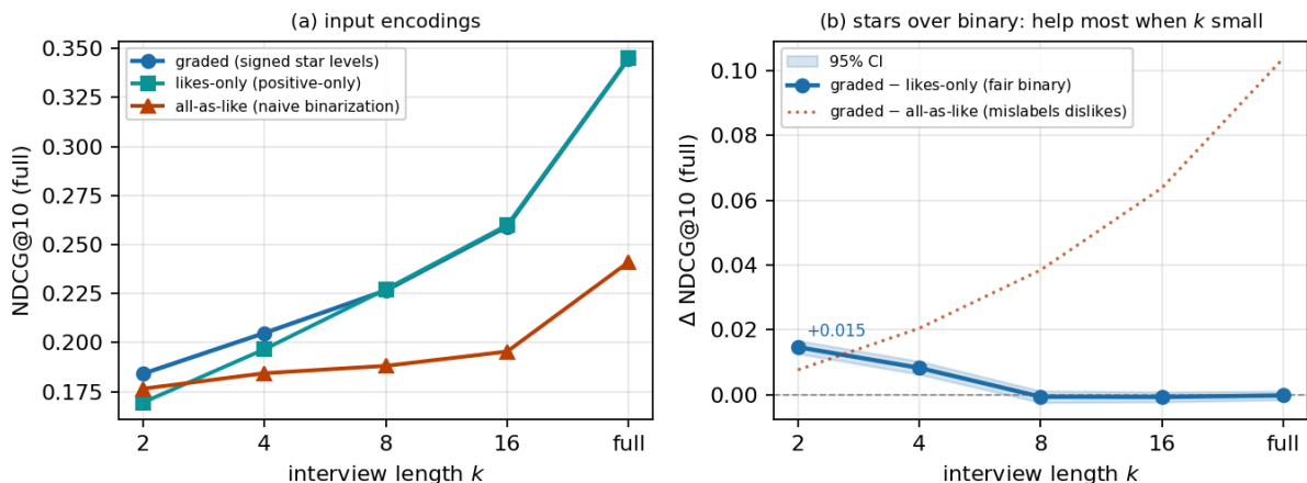
Figure 2: Graded input helps over binarized input, most on the short interview (ML-25M interview harness, full NDCG@10 vs. interview length k ). The same revealed set is fed three ways: graded (real signed star levels), likes-only (sub-threshold answers dropped—exactly what a positive-only tower such as RecVAE does at r > 3.5 ), and all-as-like (every answered item recorded as a 4-star like—naive implicit binarization). (b) Against the fair positive-only baseline, the graded premium is CI-clean positive on the short interview —+0.0147 at k=2 (CI [+0.0127, +0.0167]), +0.0083 at k=4 (CI [+0.0063, +0.0103])—and fades to a tie from k=8 onward (−0.0006, CI [−0.0024, +0.0012]) as collaborative signal fills in: the extra bits a star carries are most decisive when few items are known. The mechanism is that a signed answer encodes a dislike (a negative y_j the item-indicator basis cannot express); against the all-as-like control, which mislabels dislikes as likes, the apparent premium instead grows with k (dotted)—a control artifact (more revealed items \Rightarrow more dislikes corrupted), not value from gradation. Mirroring the star signs (flip) costs up to −0.29.
