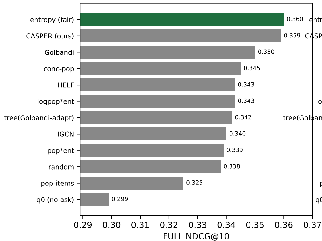
Elicitation askers on the FAIR ruler (te[300:], seed-avg) — policy vs the strong divisiveness heuristic
