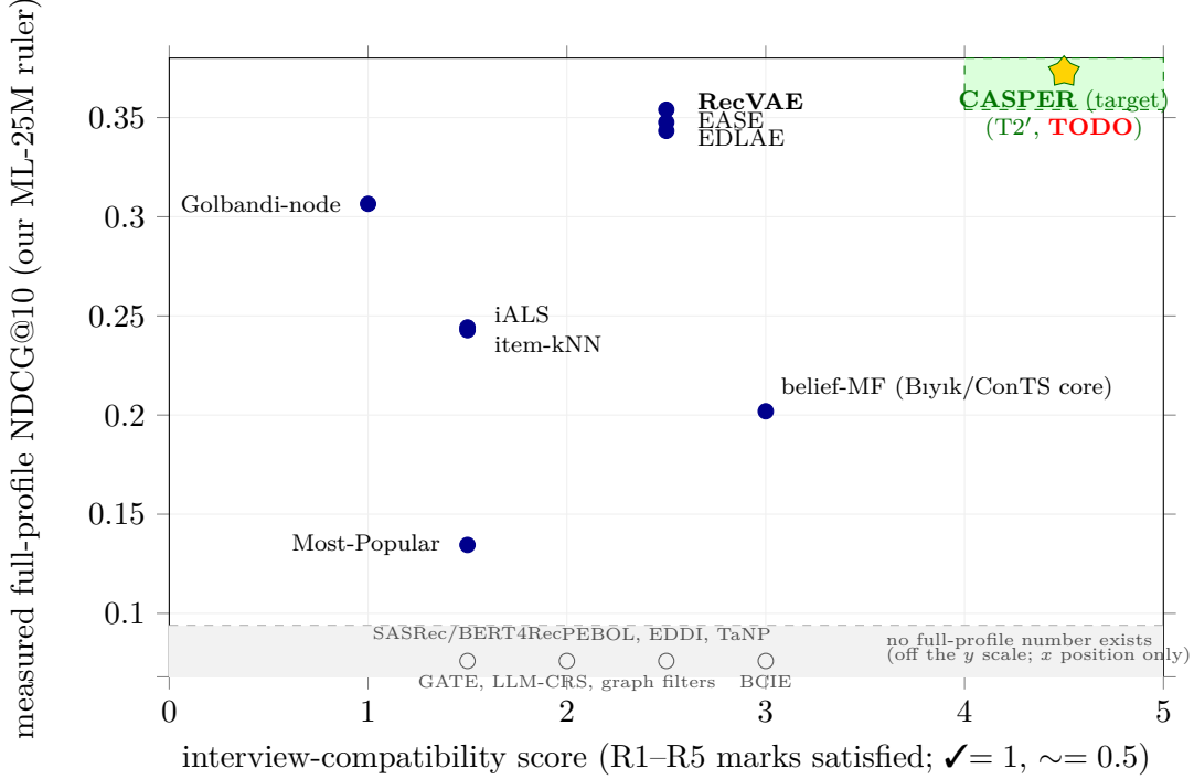
Figure 1: The gap map (measured axes). y -axis: measured full-profile NDCG@10 on our canonical ML-25M ruler. x -axis: an interview-compatibility score , defined as the number of R1–R5 marks a system carries in the master table (Table 3), scoring ✓=1 and ~.=0.5. This score is a coarse ordinal capability count , not a measurement , so the x -axis is qualitative even though the y -axis is measured. Filled markers are systems with a full-profile number on this ruler (belief-MF is the shared Bıyık/ConTS posterior core; Golbandi-node is the tree’s best-effort node recommender). Hollow markers sit in the separated grey strip below the measured y -scale: these are systems for which no full-profile number exists —unrun, unrunnable at full catalogue, or not portable (see the master-table dispositions); only their x position is meaningful. The shaded top-right box is the instrument target ( x \geq 4 and full-profile at the frontier bar), still [TODO: ] . The shape of the evidence is a collapse , not a gradual trade-off : the upper envelope is roughly flat up to the item-only accuracy corner ( x=2.5 : RecVAE/EASE/EDLAE at 0.343–0.354), then falls off a cliff — the only measured system beyond it (belief-MF at x=3.0 ) drops to 0.2019, below plain matrix factorisation, and nothing measurable exists at x \geq 3.5 . The corner is not expensive; it is unoccupied. The nearest published rival to the target is Bıyık et al. [2] (highest compatibility of any system with an actionable belief), whose runnable core nonetheless measures at 0.2019 full—far below the frontier bar.
