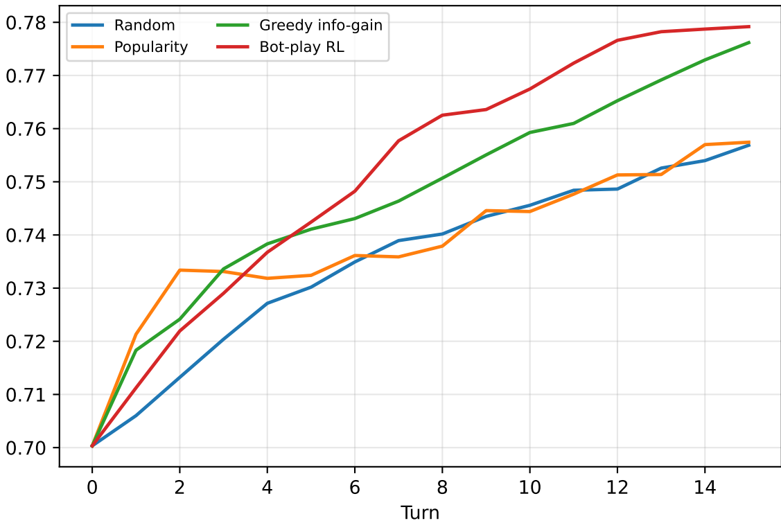
Mean accuracy on held-out ratings
