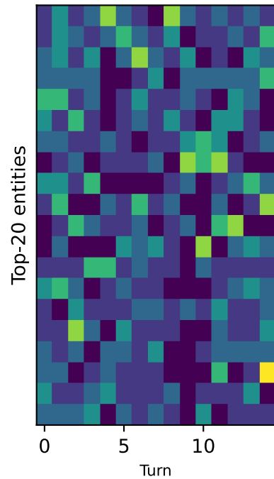
Random
