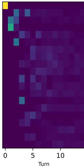
Greedy info-gain
