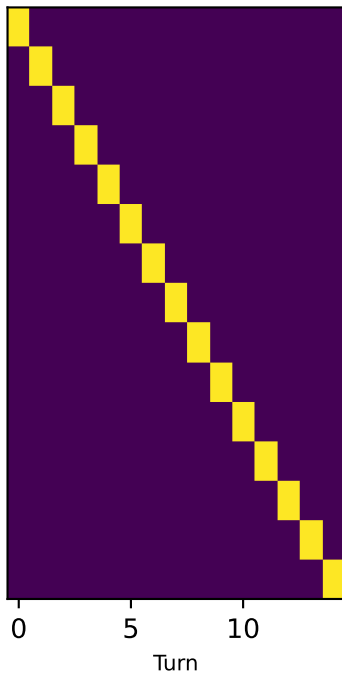
Popularity
