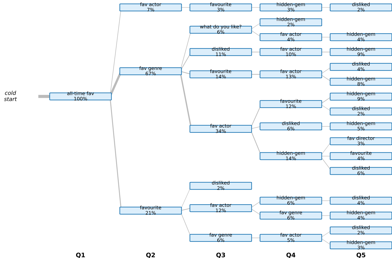
Learned question tree (greedy policy; % = users reaching node)
