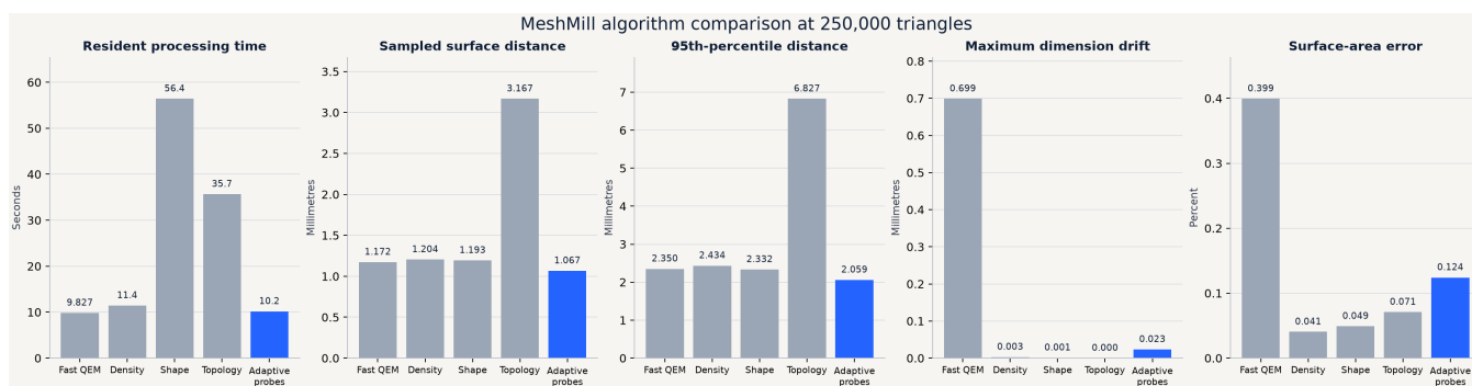
Runtime and geometry-error comparison
