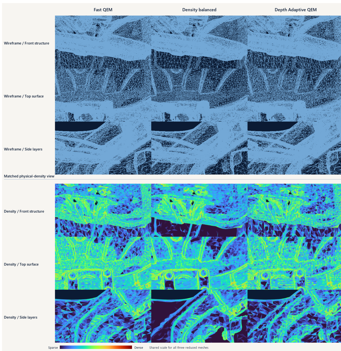
Single-page matched comparison of Fast QEM, Density balanced, and Depth Adaptive QEM in close wireframe and physical-density views
