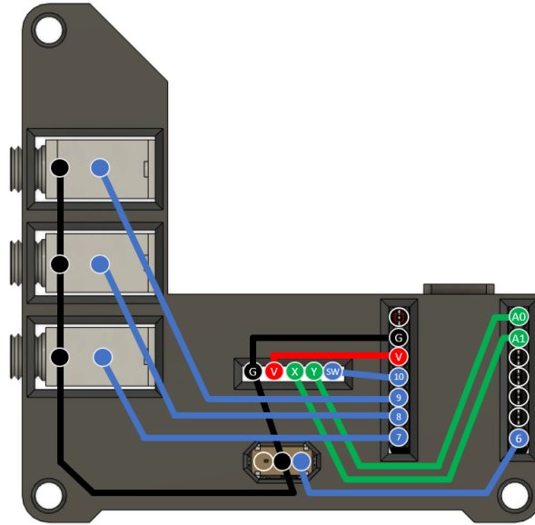
Figure 1. Joystick Wiring Guide
