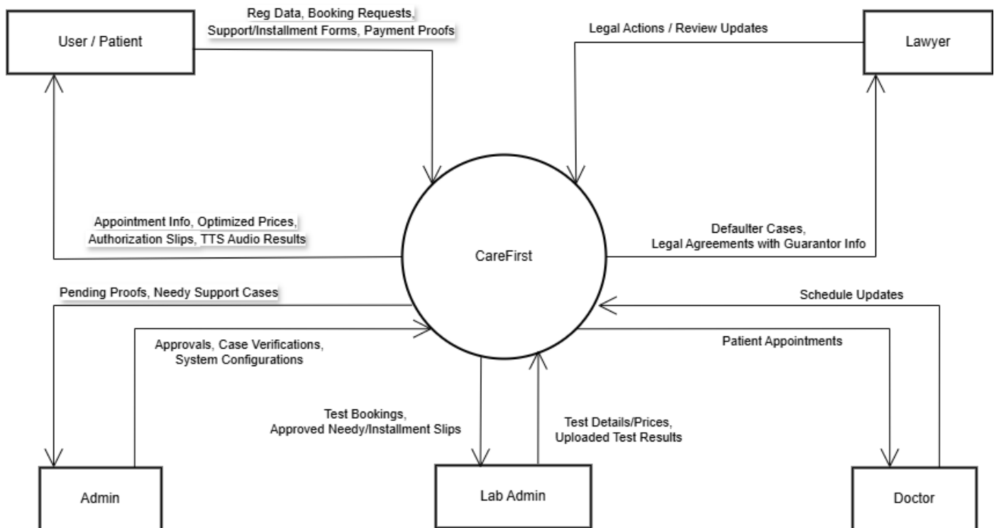
figure 28: DFD Level 0
