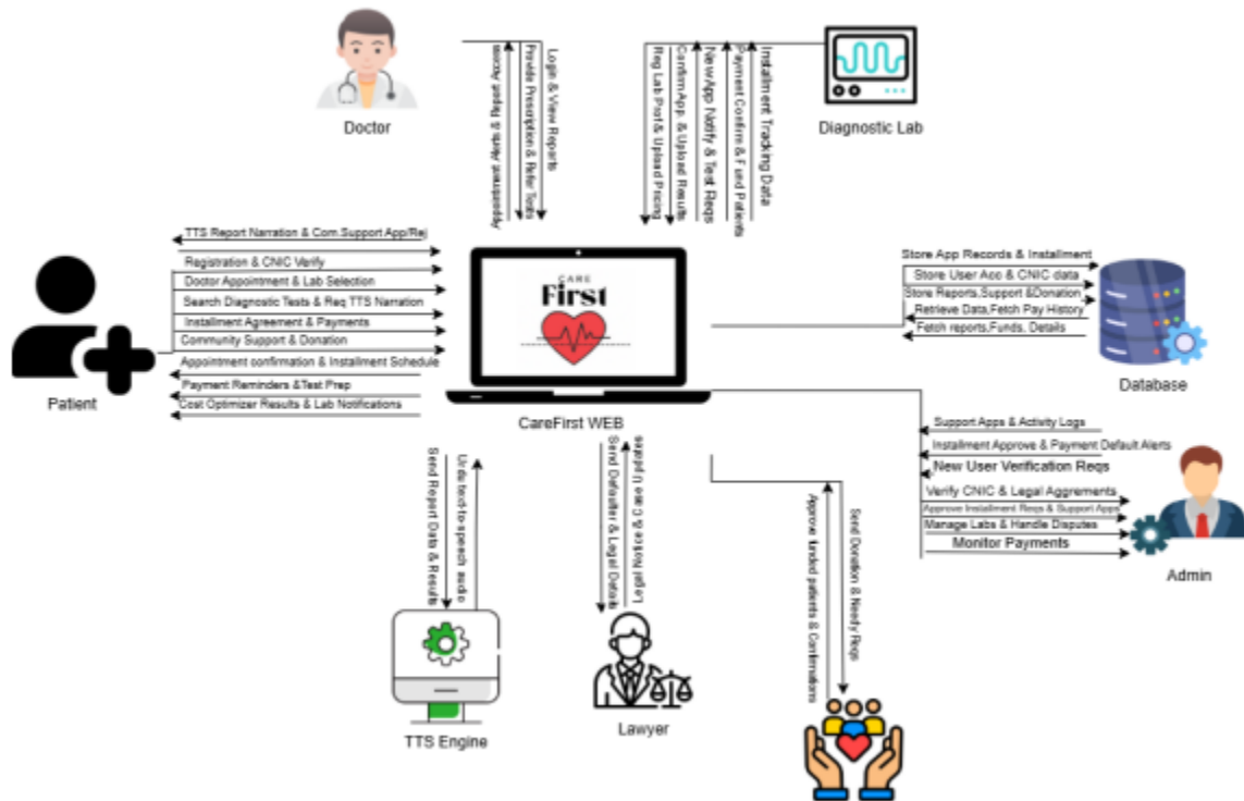
Figure 35: Architecture Diagram
