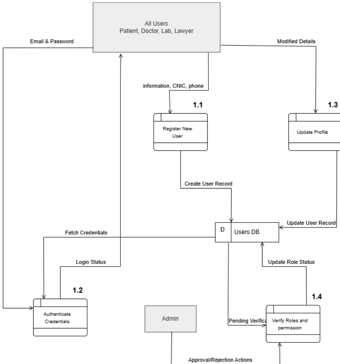
figure 30: Manage Users
