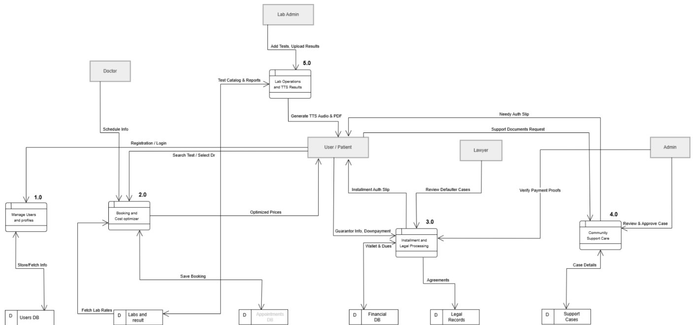
figure 29: DFD Level 1
