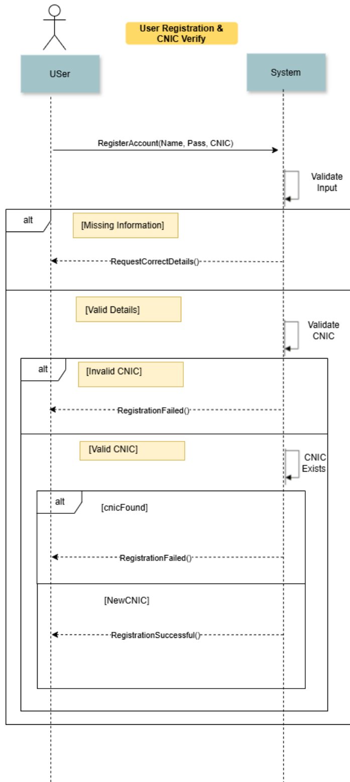
Figure 13: User Login/Register
