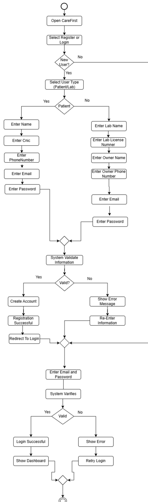
Figure 2: Register/Login
