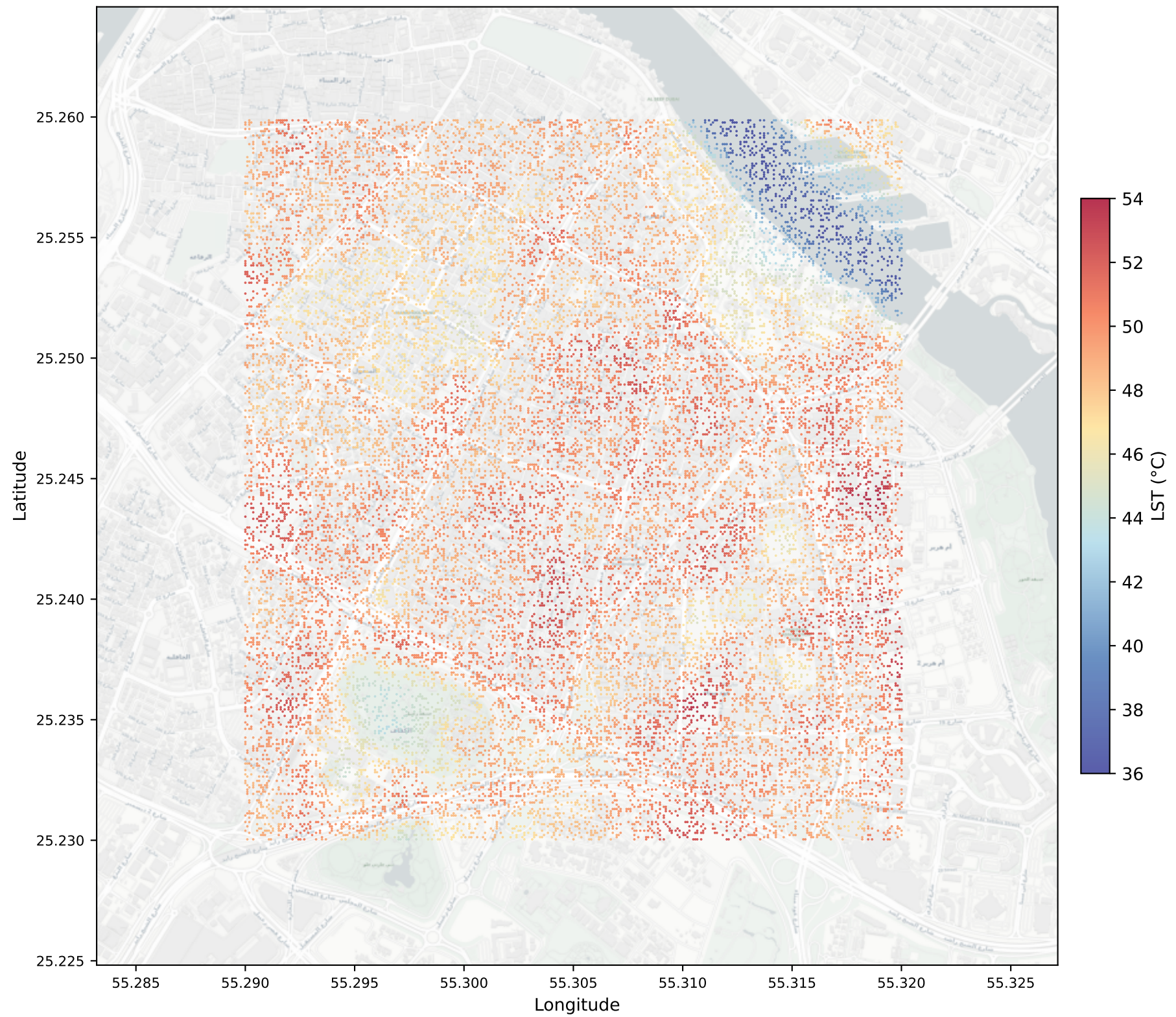
Satellite Grid - Land Surface Temperature (30m)
