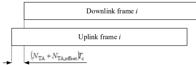
Figure 4.3.1-1: Uplink-downlink timing relation.
