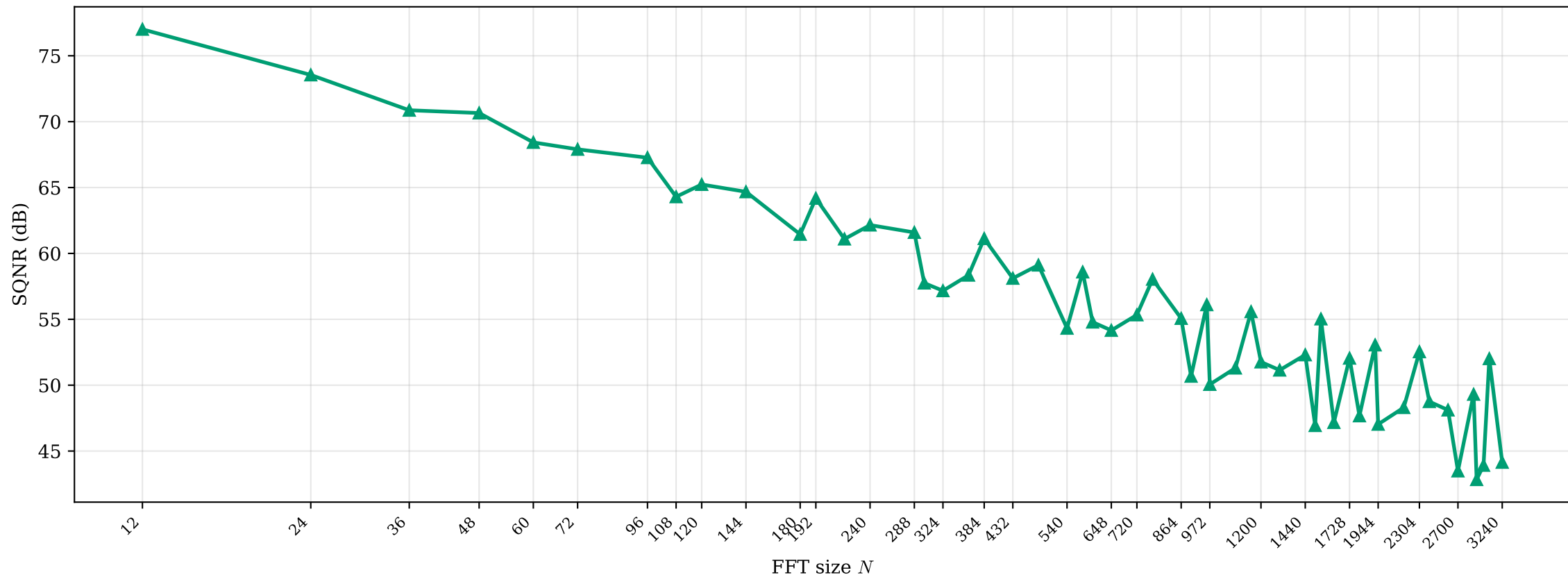
SQNR vs FFT size
