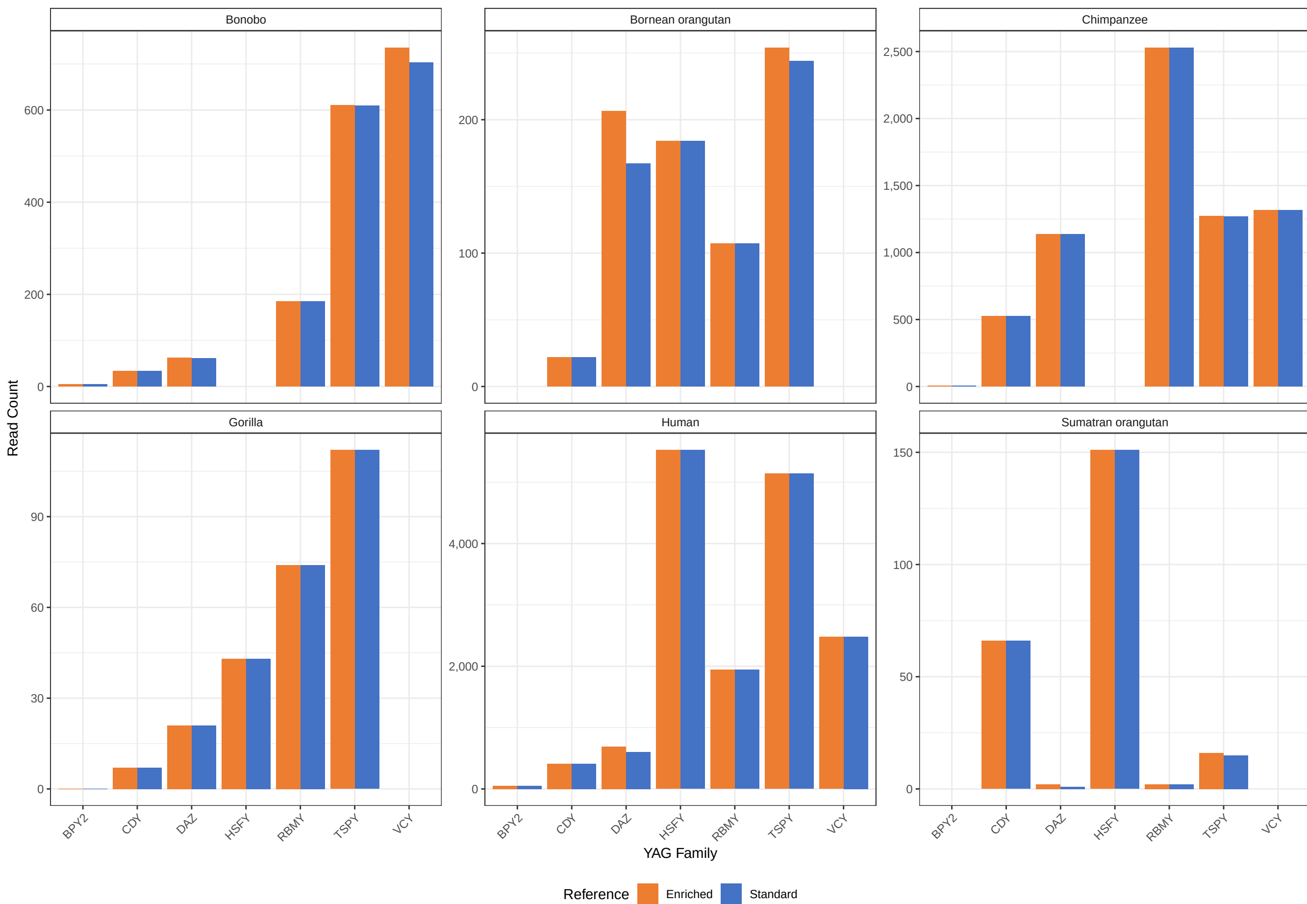
YAG Read Counts: Standard vs Enriched Reference
