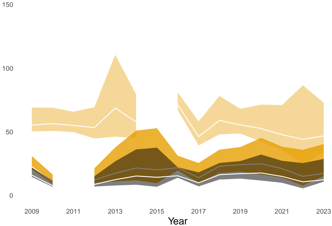
Sex-specific populations size
