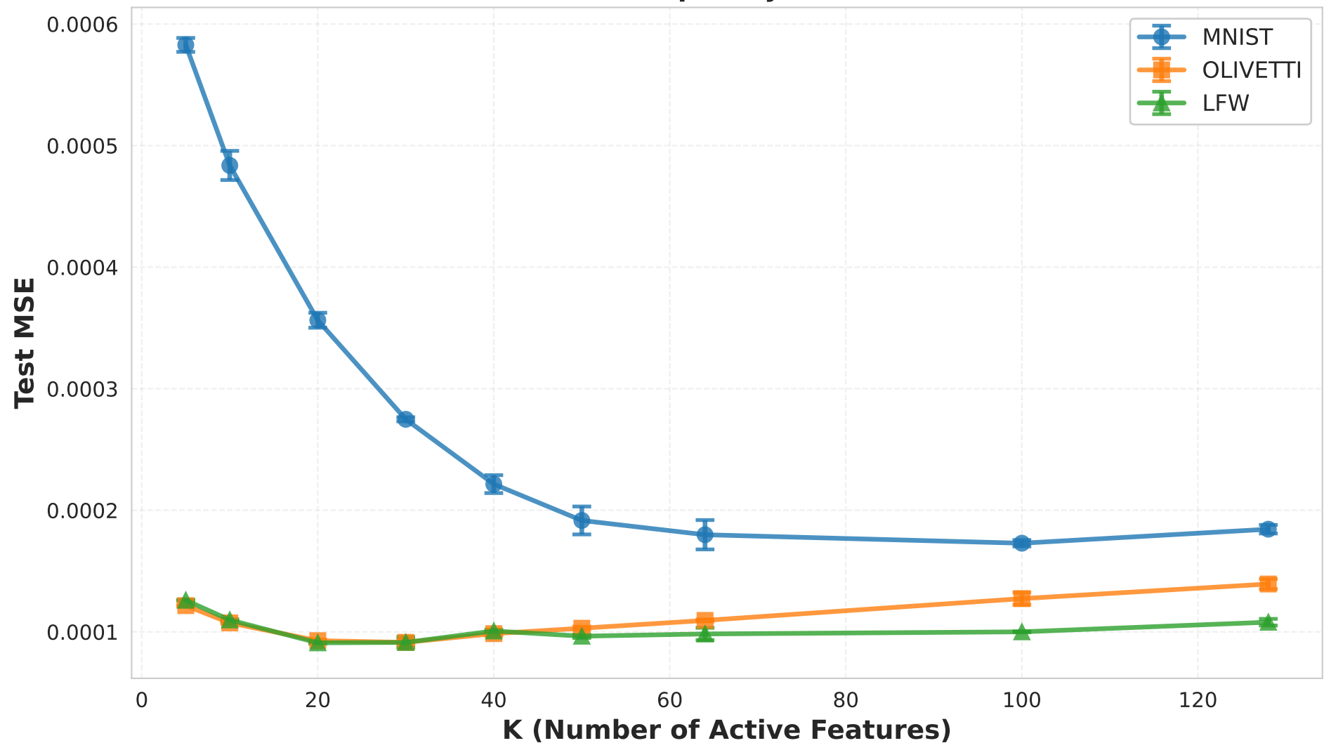
Reconstruction Error vs Sparsity Level (Hidden Size=256)
