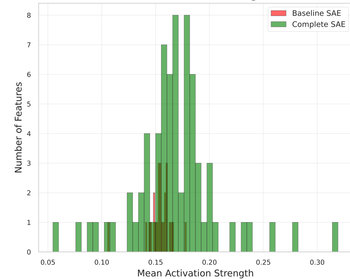
MNIST: Activation Strengths
