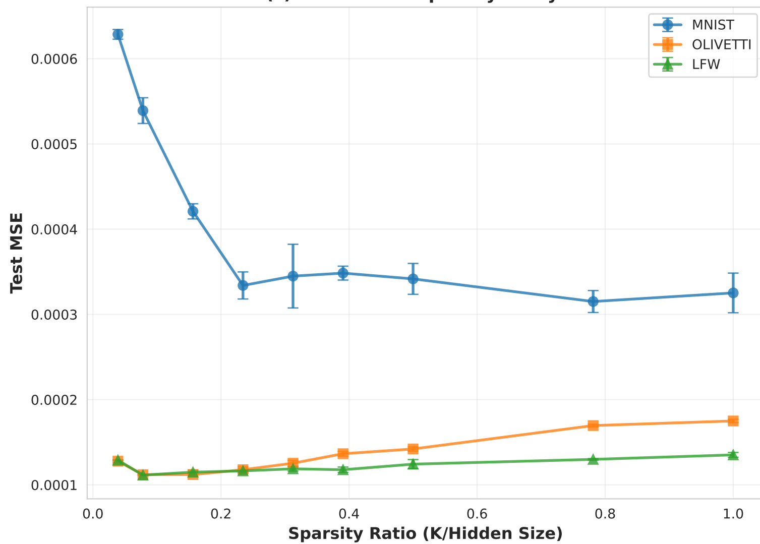
(c) Normalized Sparsity Analysis
