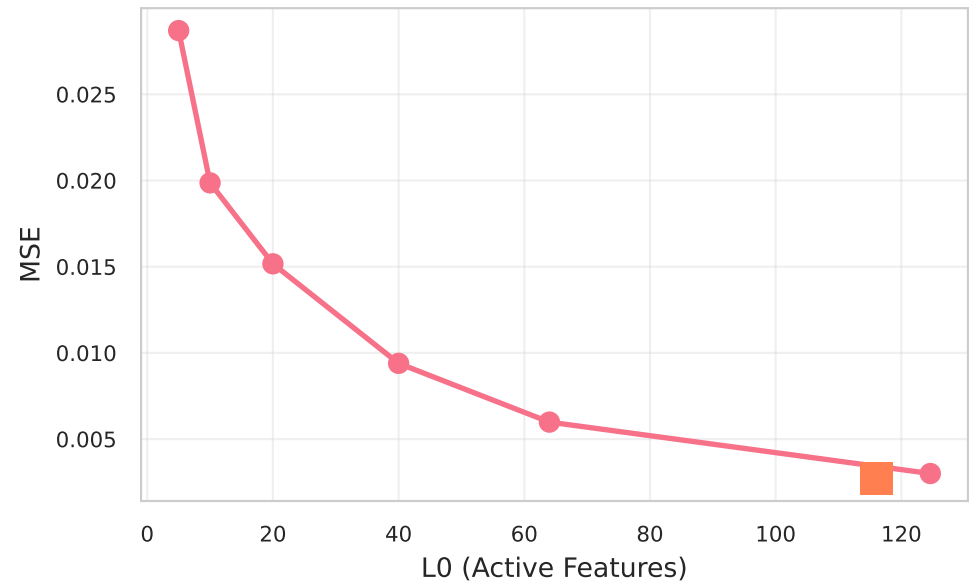
MNIST: Interpretability
