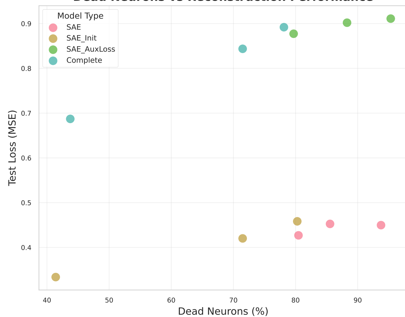
Dead Neurons vs Reconstruction Performance
