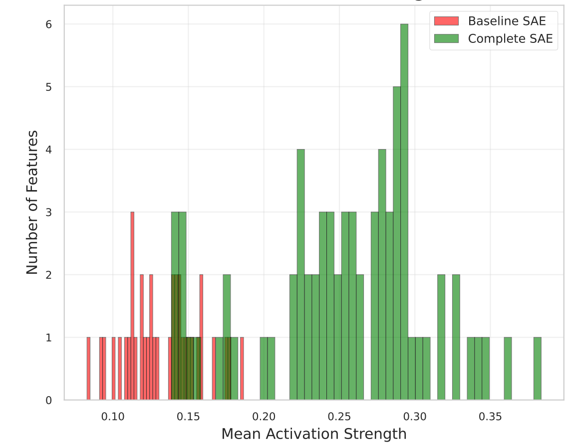
OLIVETTI: Activation Strengths
