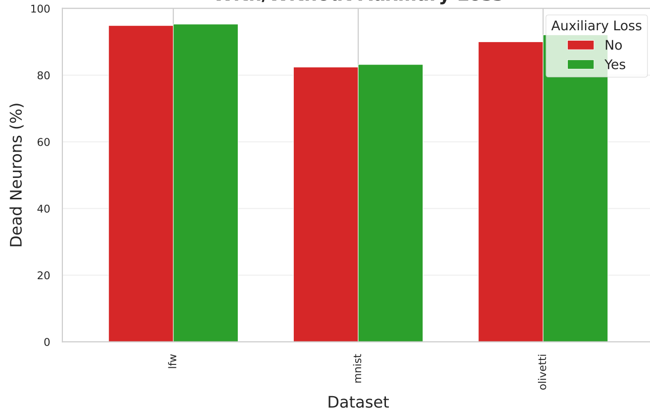
Dead Neuron Percentage With/Without Auxiliary Loss
