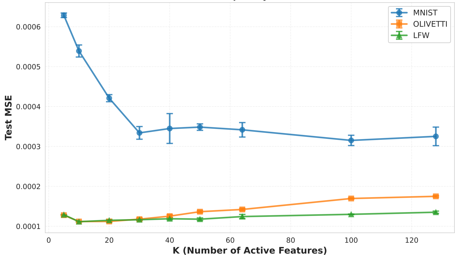
Reconstruction Error vs Sparsity Level (Hidden Size=128)
