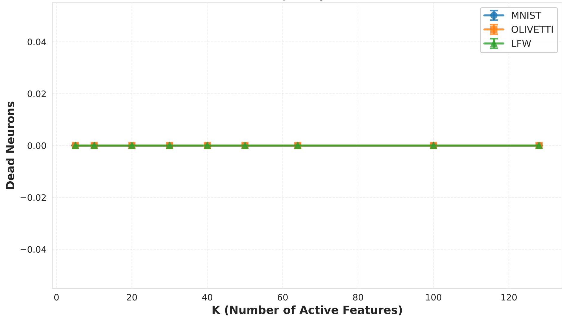
Dead Neuron Count vs Sparsity Level (Hidden Size=256)
