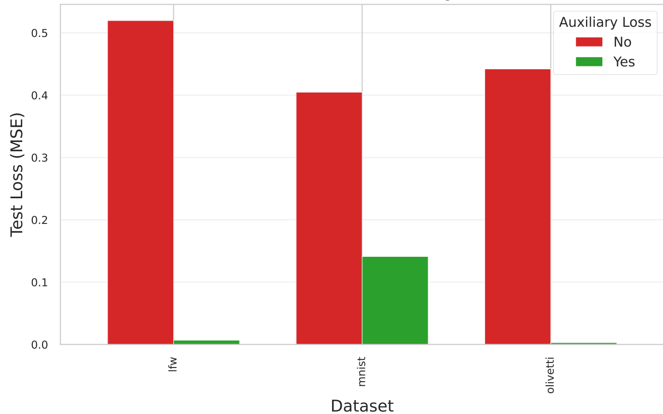
Reconstruction Loss With/Without Auxiliary Loss
