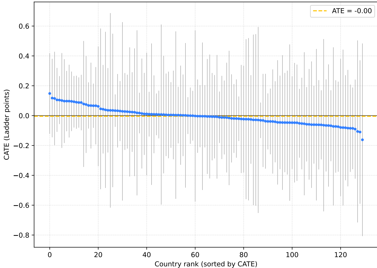
Ranked country-level CATEs with 95% confidence intervals
