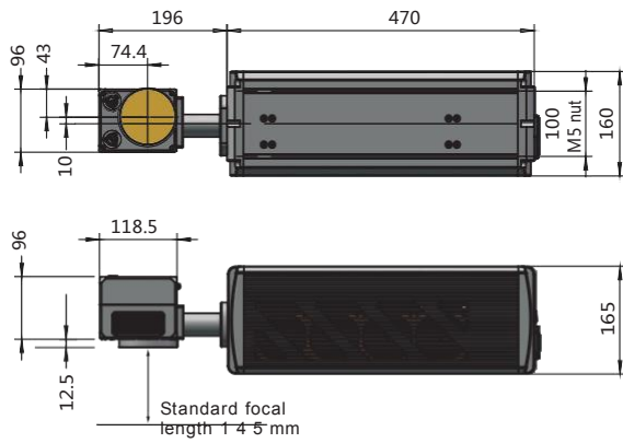
30W Laser head size:
