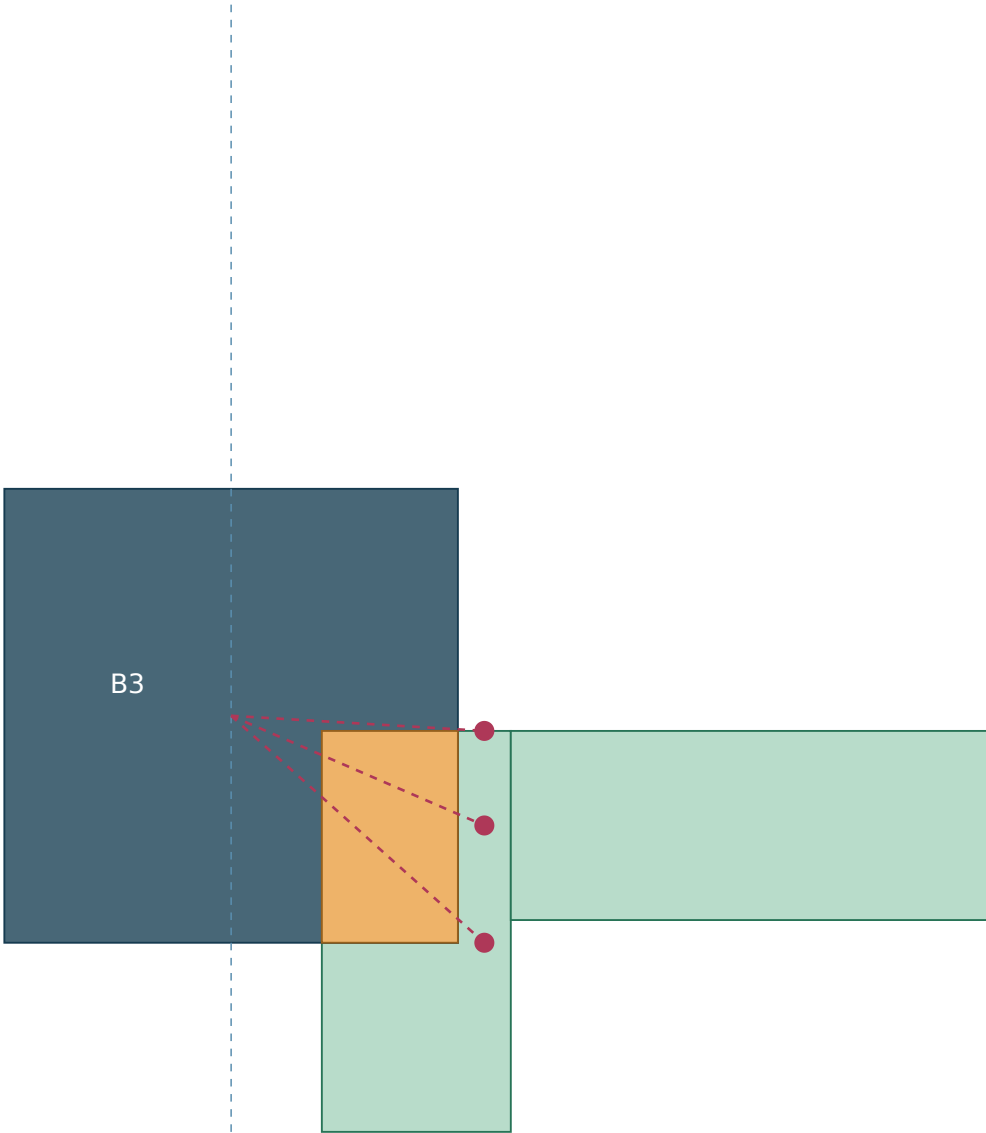
B3 PLAN / 1:10 / analytical slice z = +2.00 m
