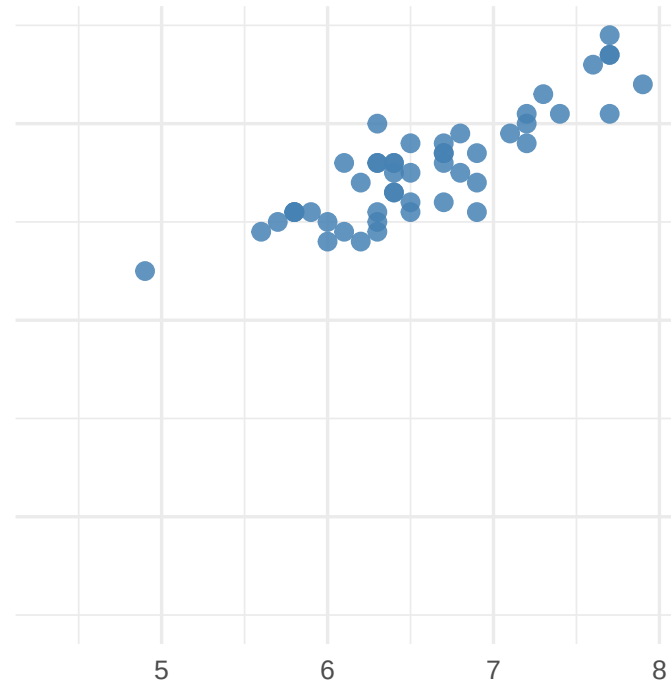
virginica
