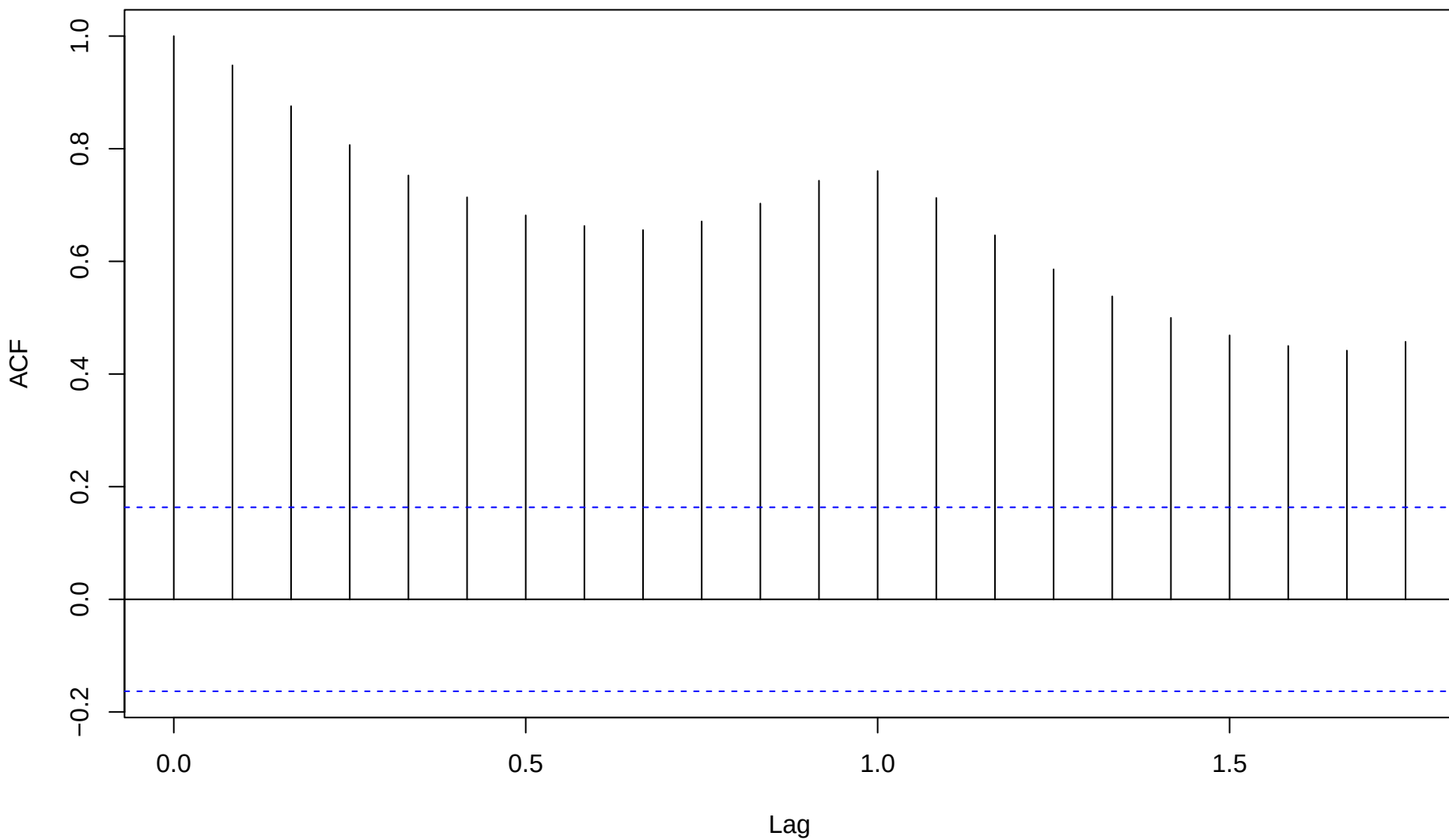
ACF: ..... AirPassengers
