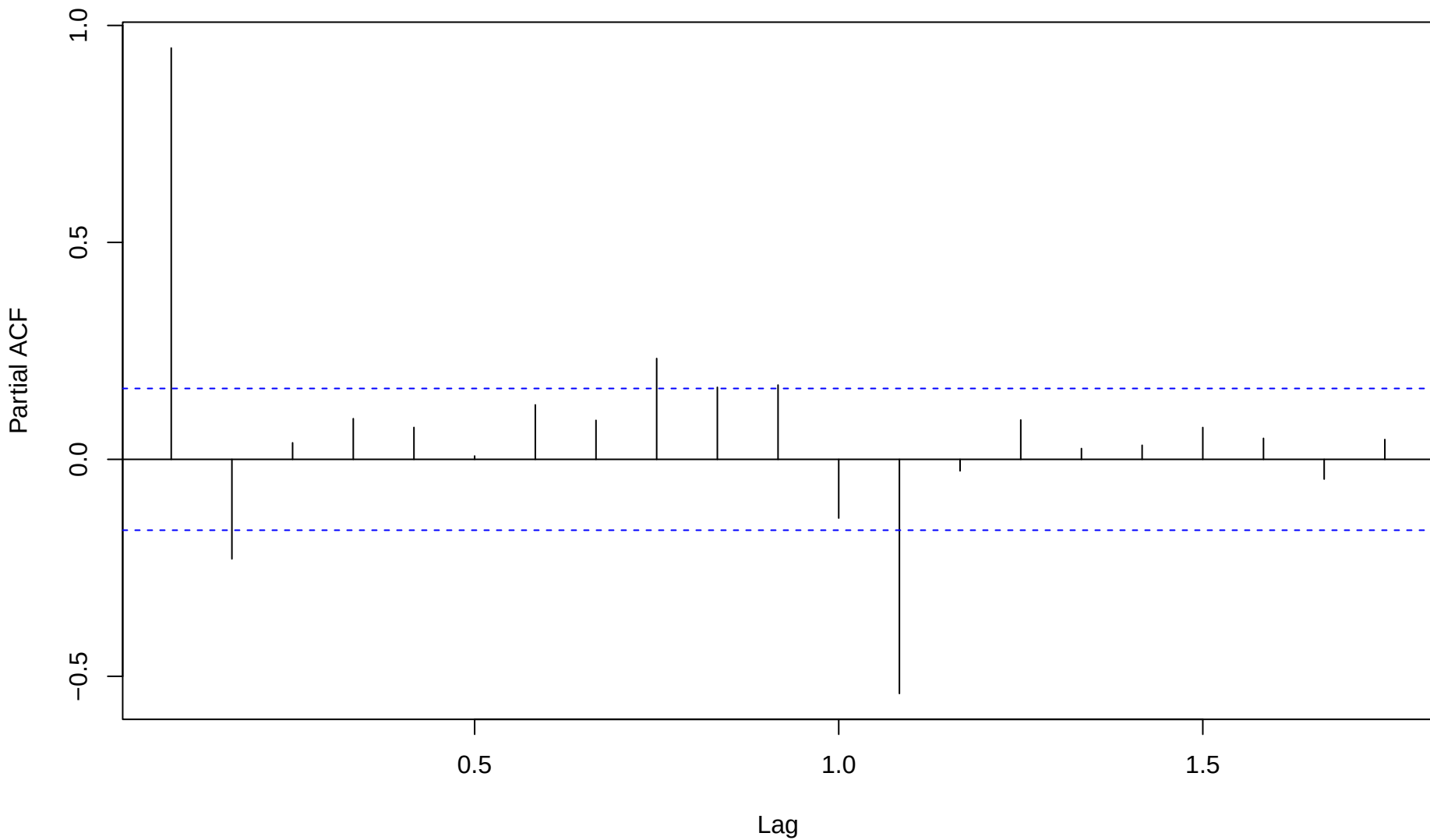
PACF: ..... AirPassengers
