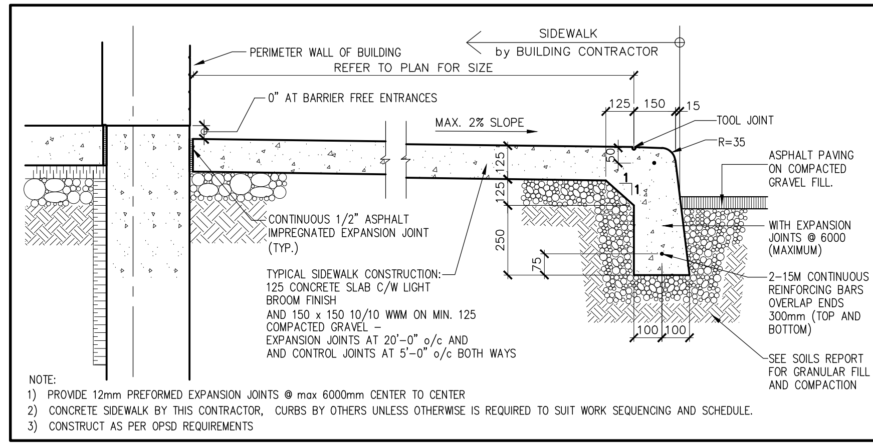
5 TYP. CONCRETE SIDEWALK DETAIL SCALE: 1" = 1'-0"
