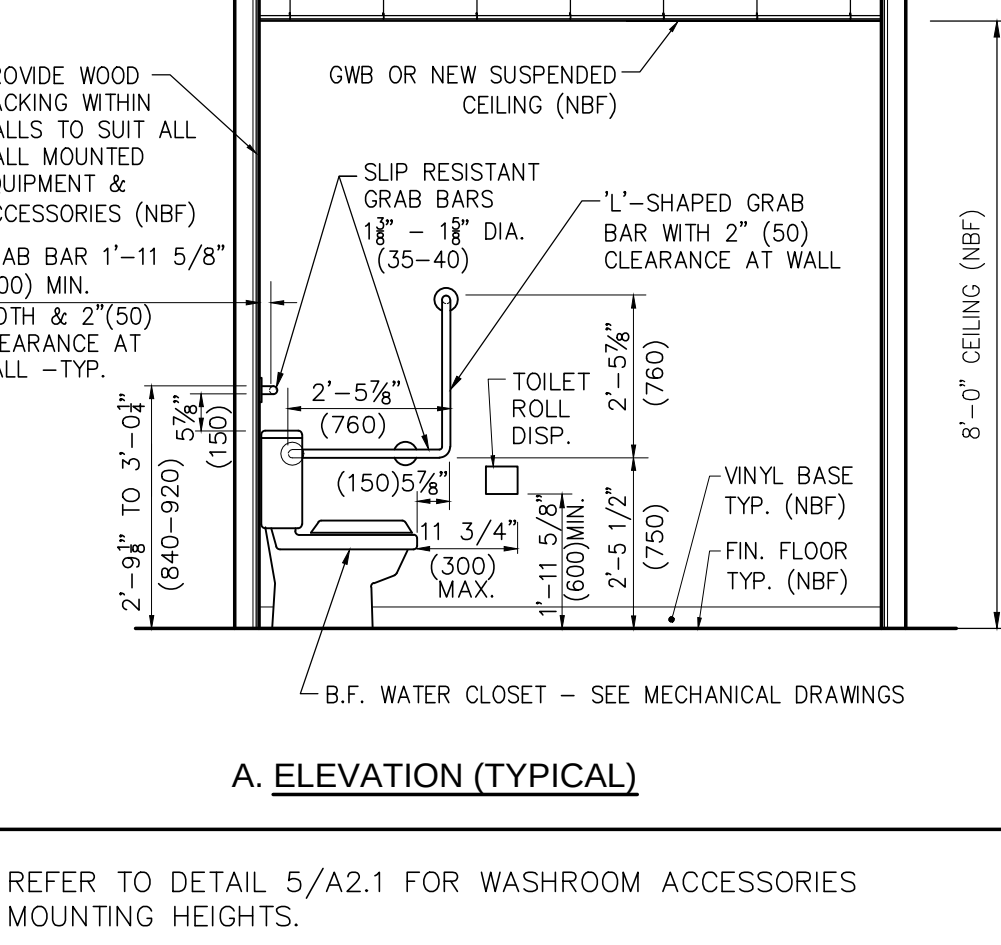
A. ELEVATION (TYPICAL) REFER TO DETAIL 5/A2.1 FOR WASHROOM ACCESSORIES MOUNTING HEIGHTS.
