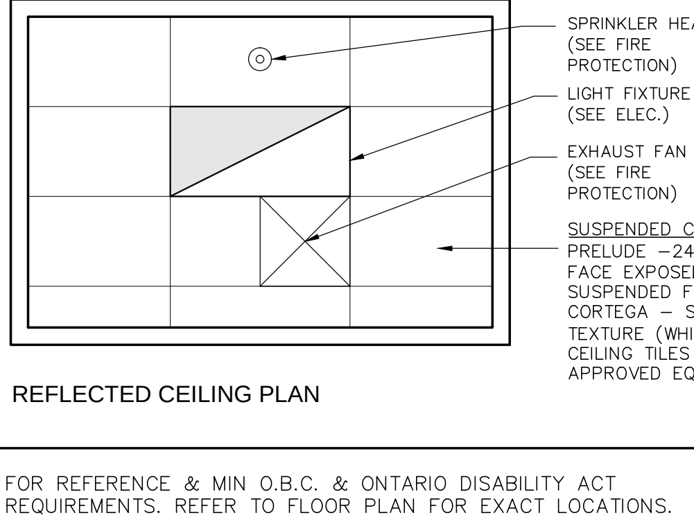
REFLECTED CEILING PLAN FOR REFERENCE & MIN O.B.C. & ONTARIO DISABILITY ACT REQUIREMENTS. REFER TO FLOOR PLAN FOR EXACT LOCATIONS.
