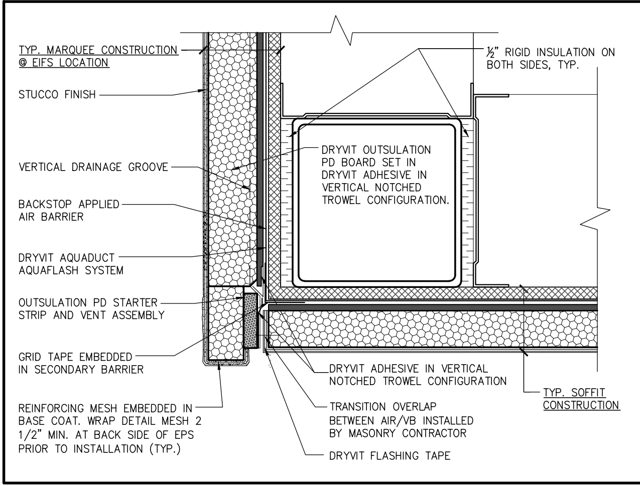
4 SECTION DETAIL SCALE: 3\"/>
