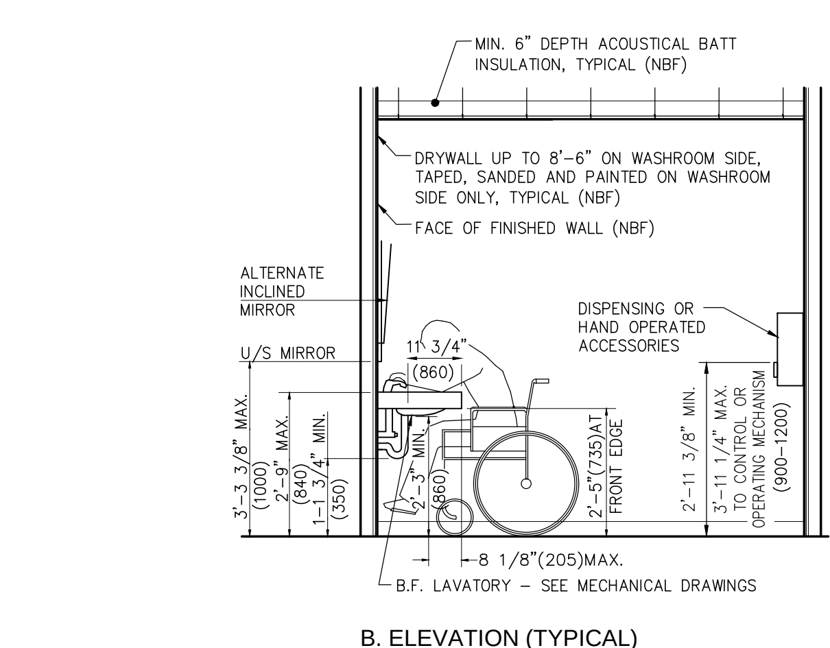
B. ELEVATION (TYPICAL) REFER TO DETAIL 5/A2.1 FOR WASHROOM ACCESSORIES MOUNTING HEIGHTS.
