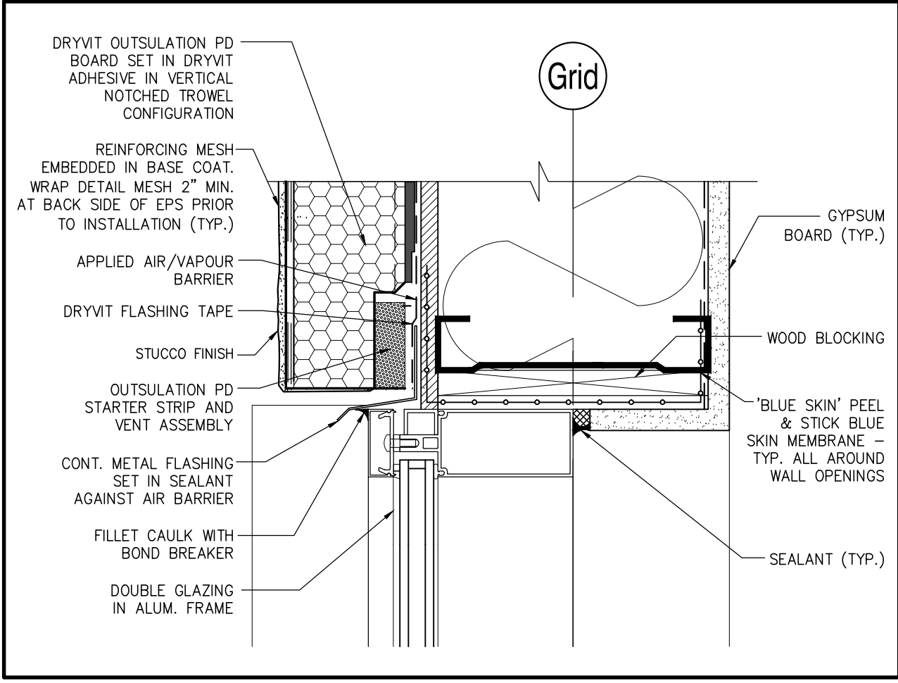
11 SECTION DETAIL SCALE: 3\"/>
