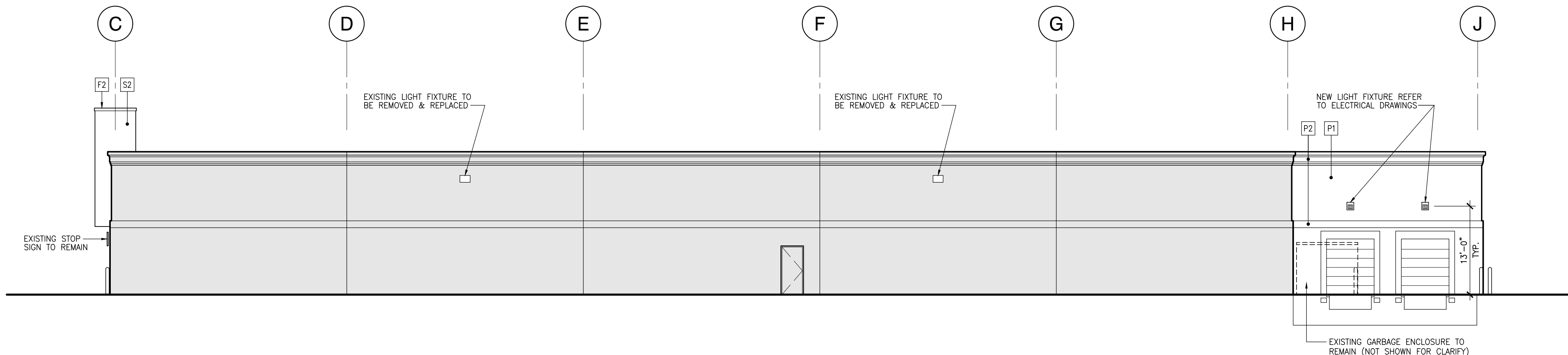
3 PROPOSED WEST ELEVATION SCALE: 3/32" = 1'-0"
