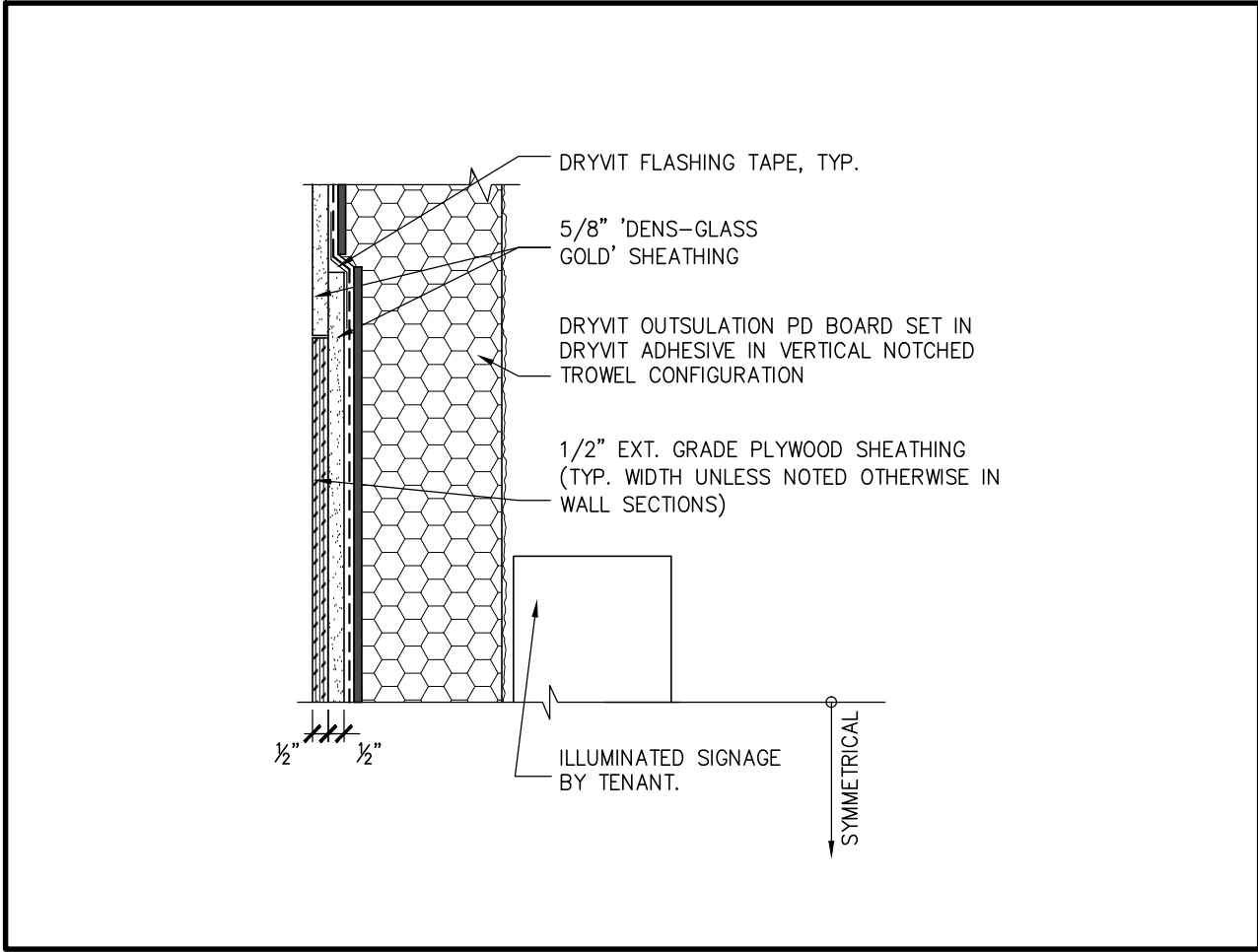
12 SECTION DETAIL SCALE: 6\"/>
