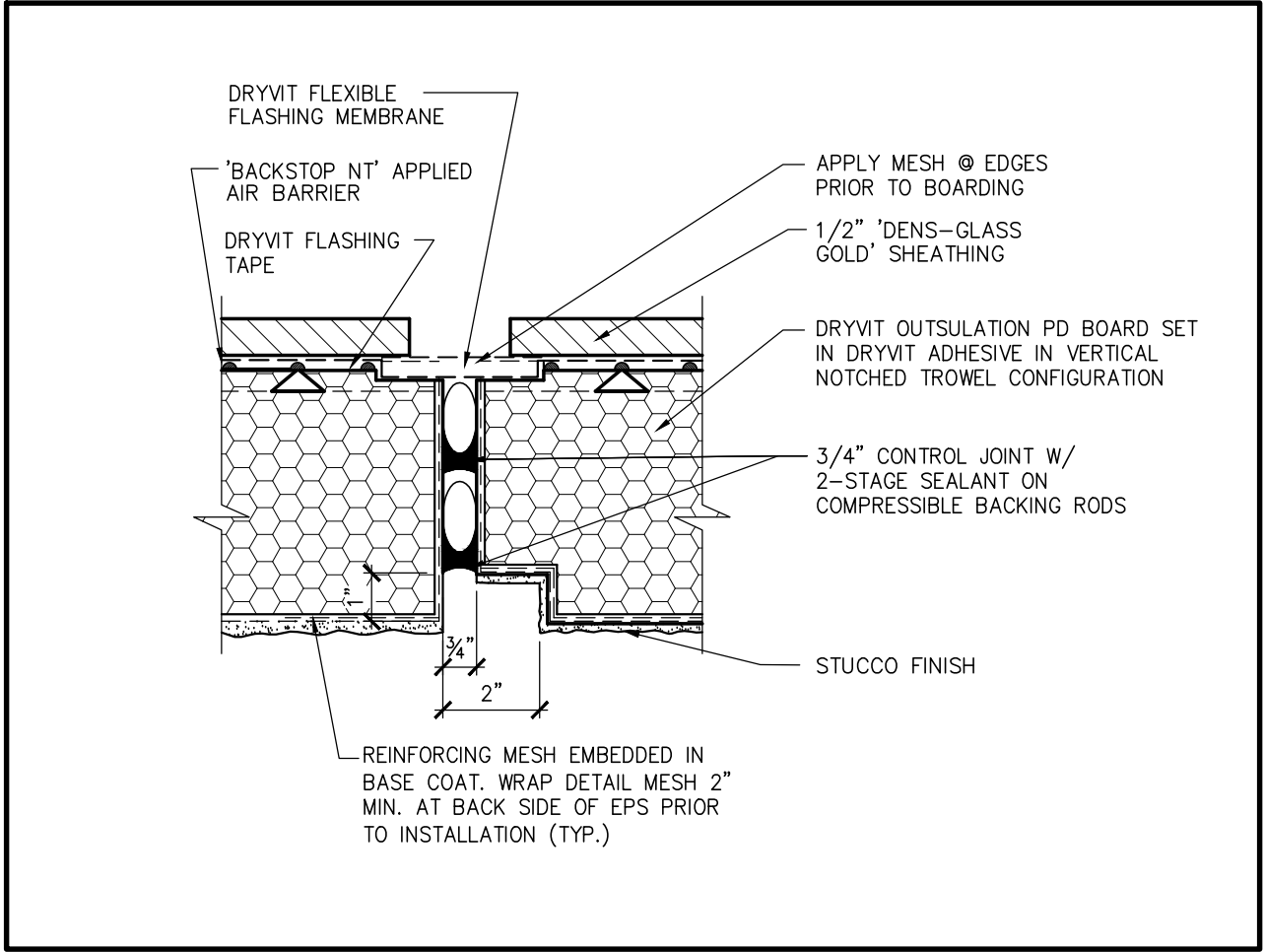
17 TYP. VERTICAL CONTROL JOINT SCALE: 3\"/>
