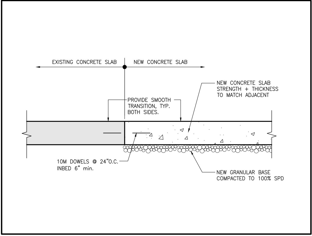
16 SECTION DETAIL SCALE: NTS
