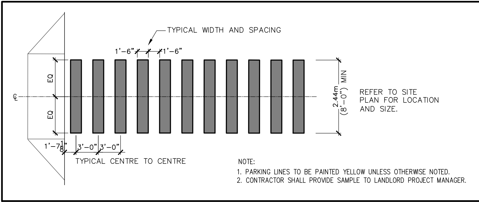
7 TYP. PAINTED CROSSWALKS SCALE: N.T.S.
