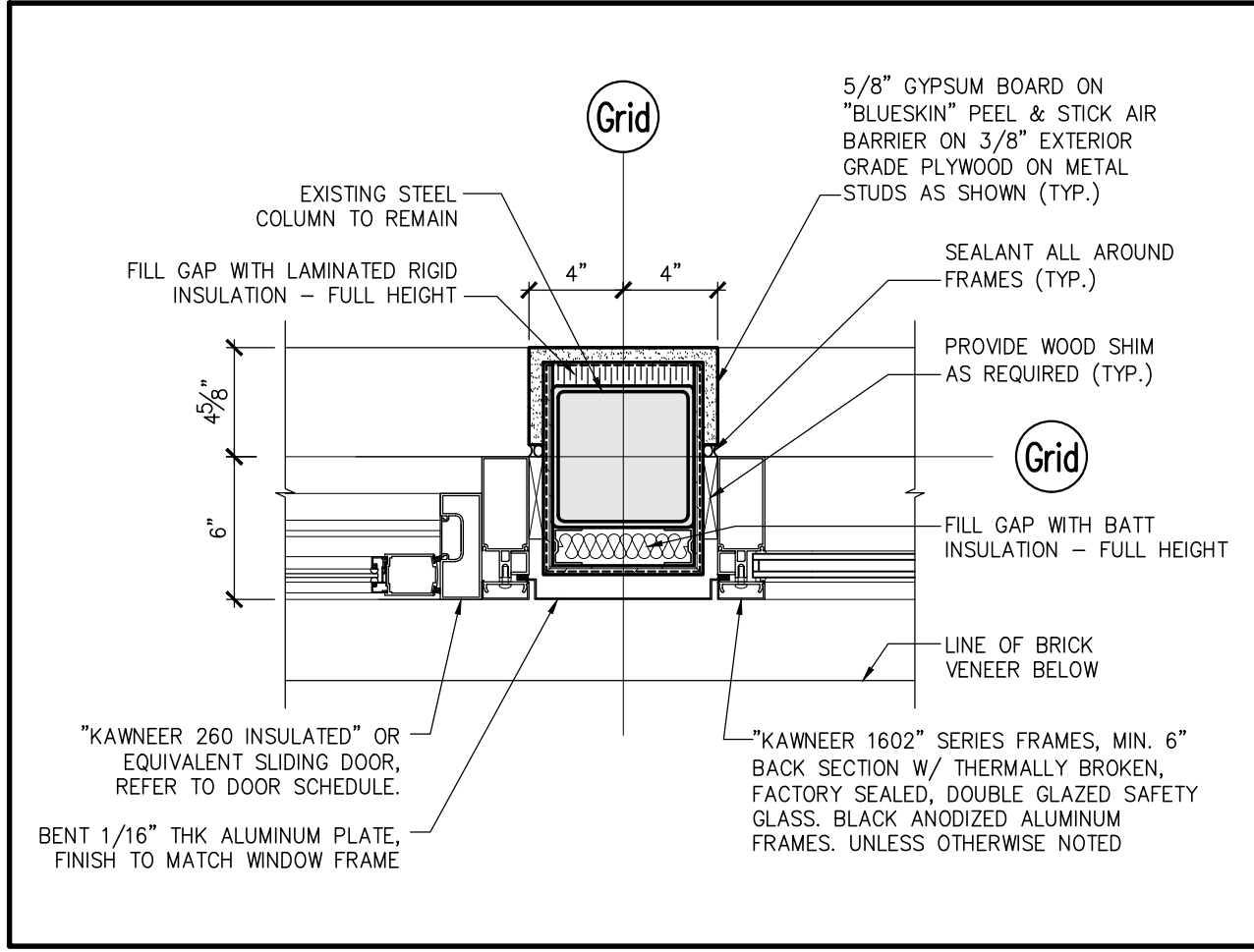
9 PLAN DETAIL SCALE: 1 1/2\"/>
