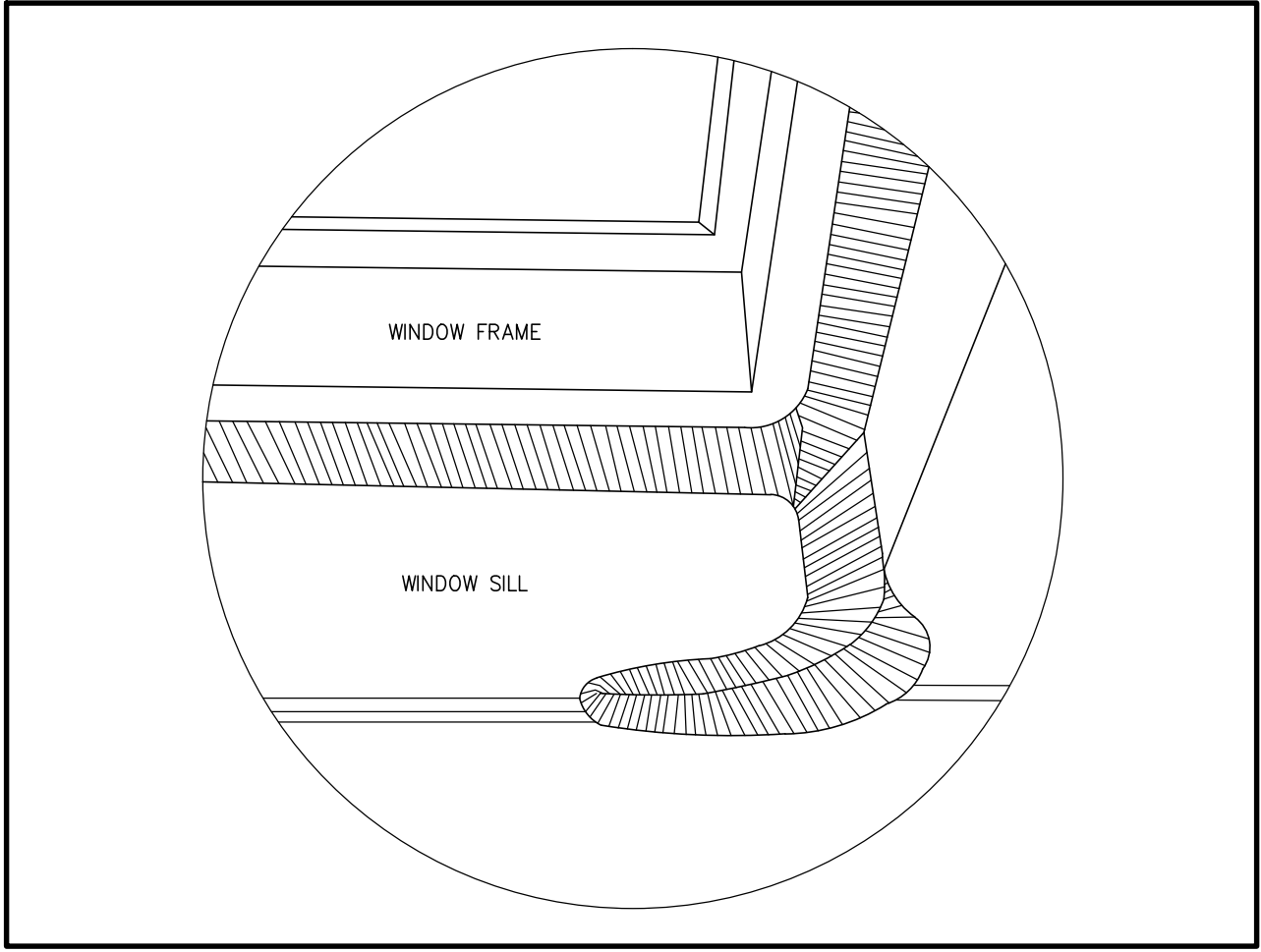
19 CAULKING DAM DETAIL SCALE: NTS
