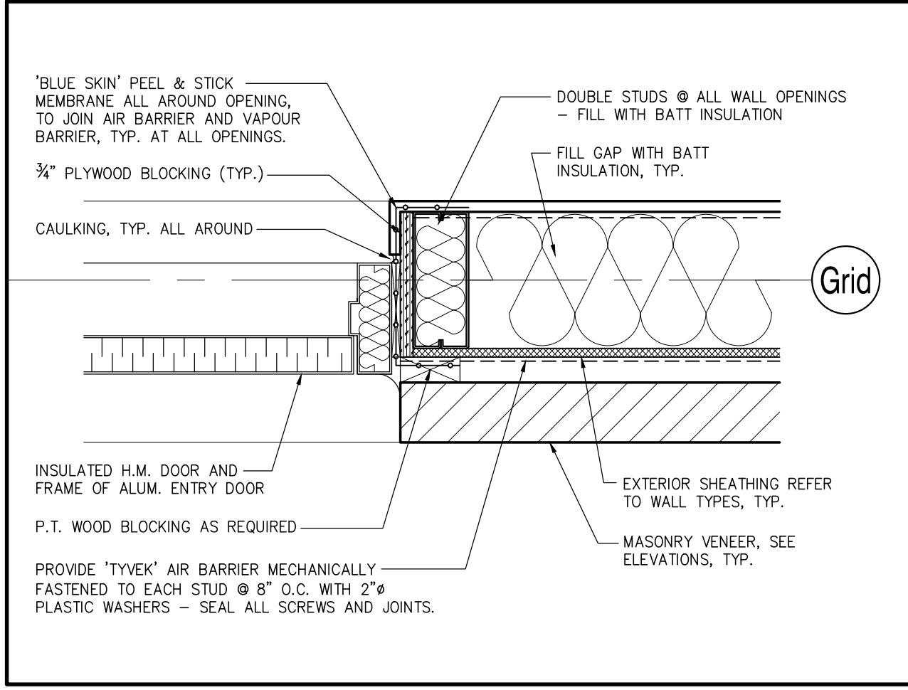
6 PLAN DETAIL SCALE: 1 1/2\"/>
