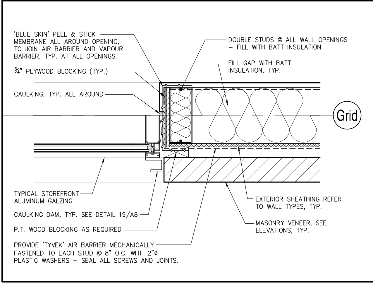
1 PLAN DETAIL SCALE: 1 1/2\"/>
