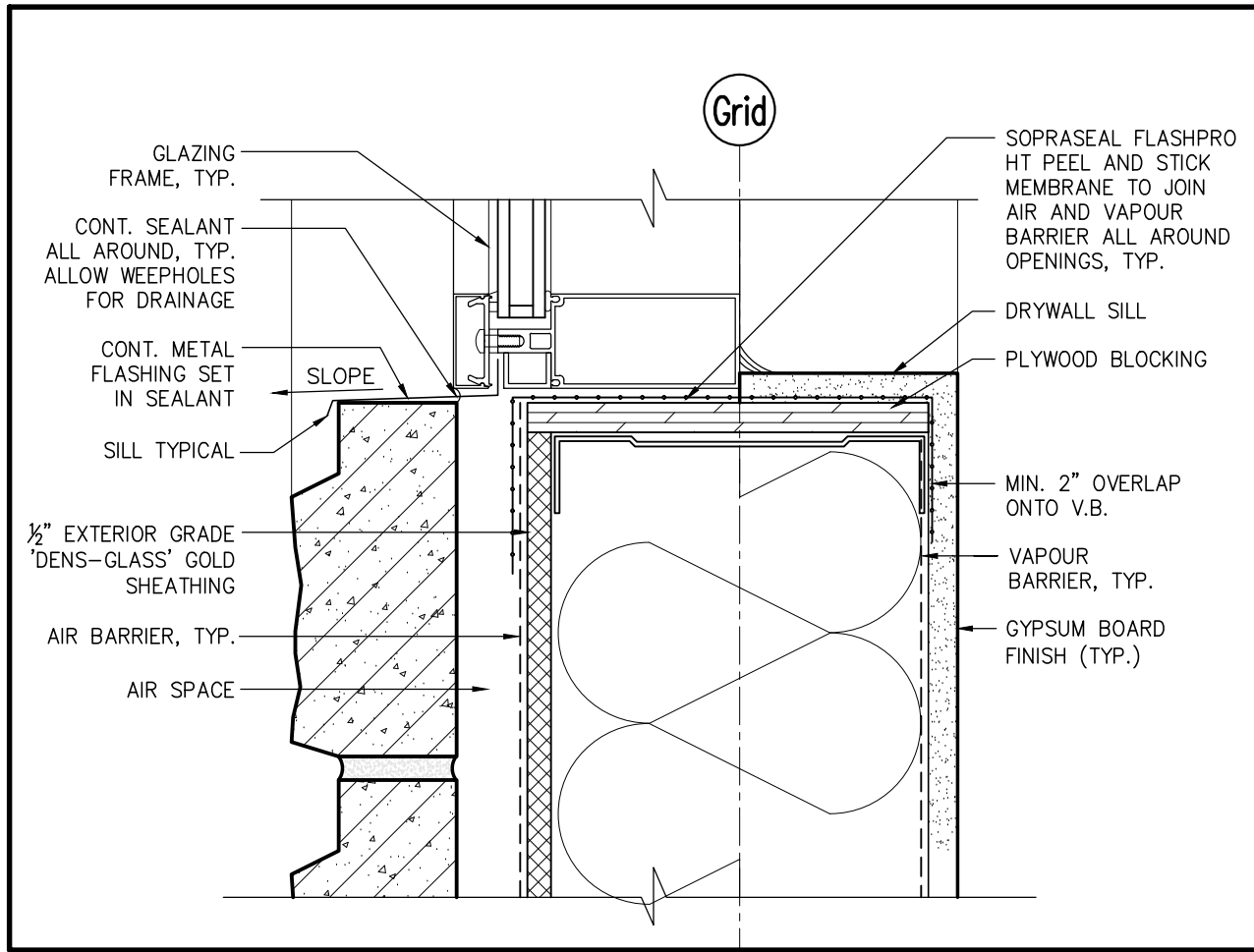
8 SECTION DETAIL SCALE: 3\"/>
