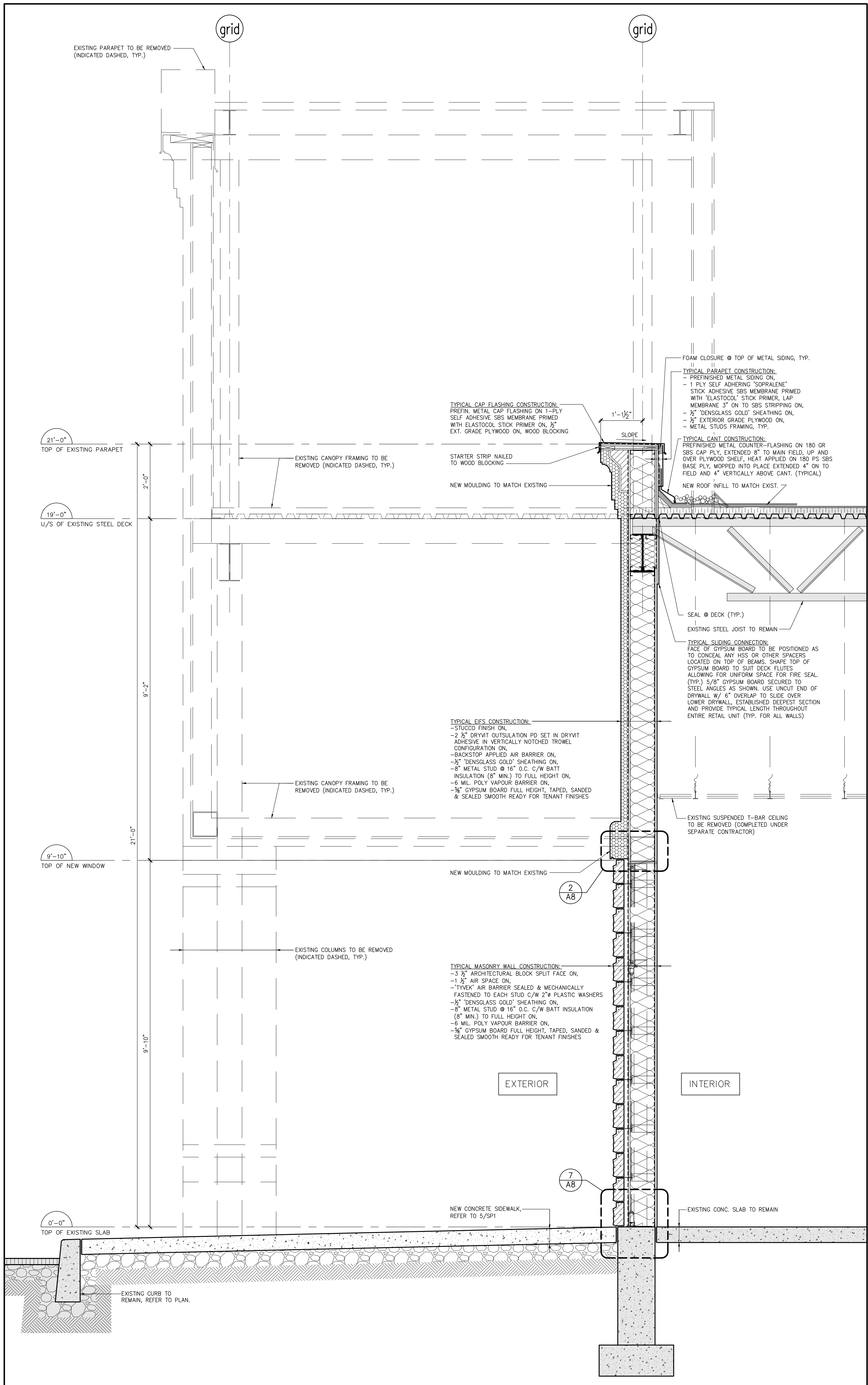
1 WALL SECTION SCALE: 3/4" = 1'-0"
