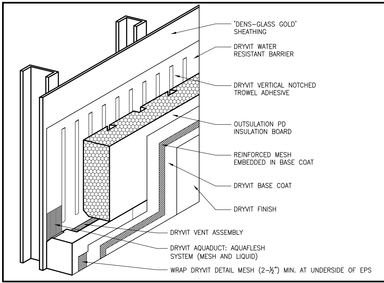
10 EIFS APPLICATION SCALE: NTS
