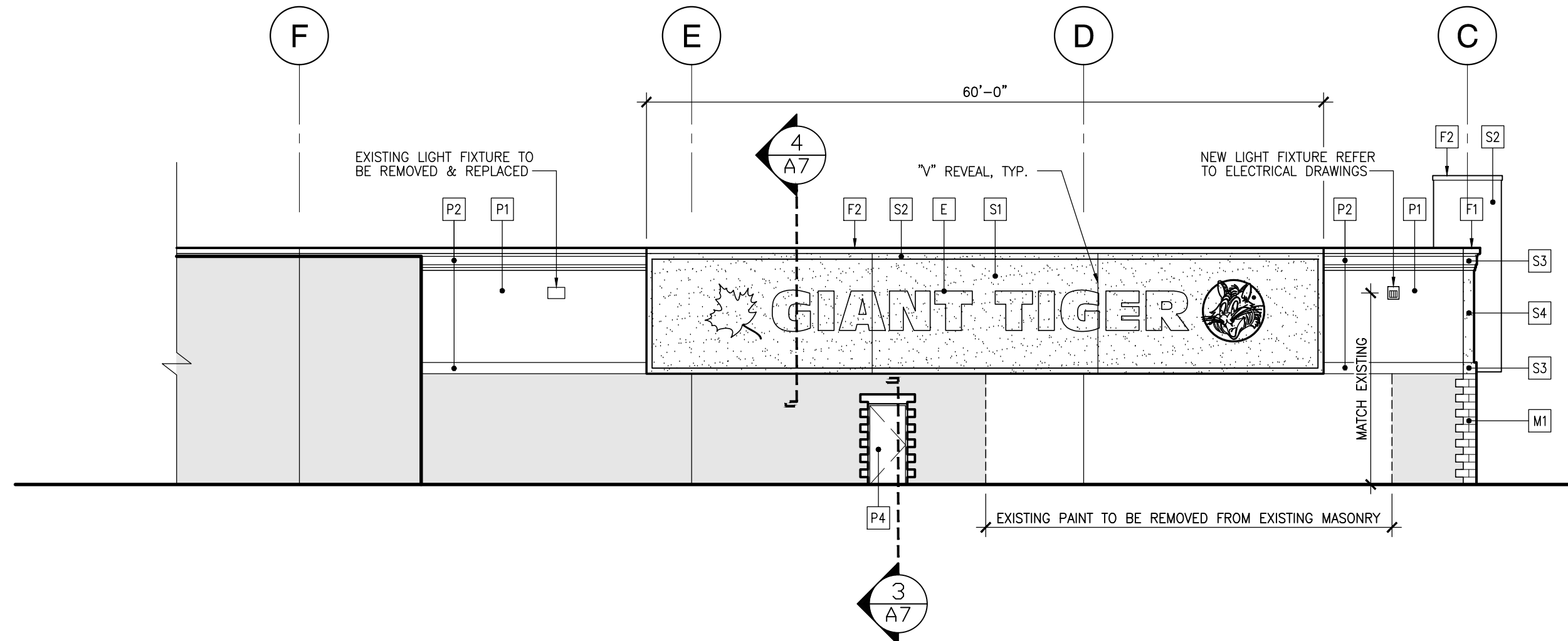
4 PROPOSED EAST ELEVATION SCALE: 3/32" = 1'-0"
