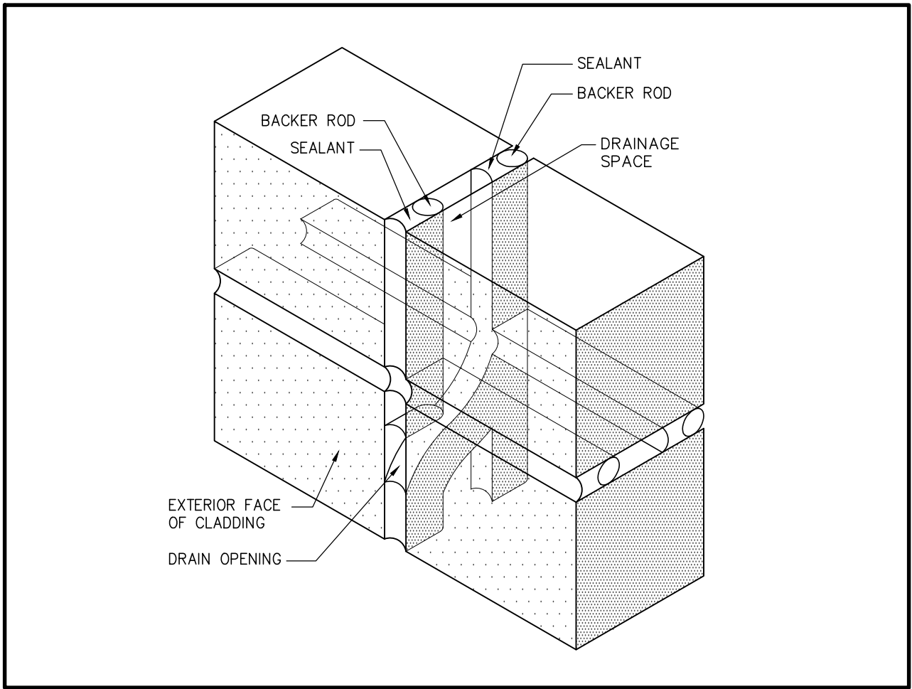
18 TWO-STAGE SEALANT JOINT SCALE: NTS
