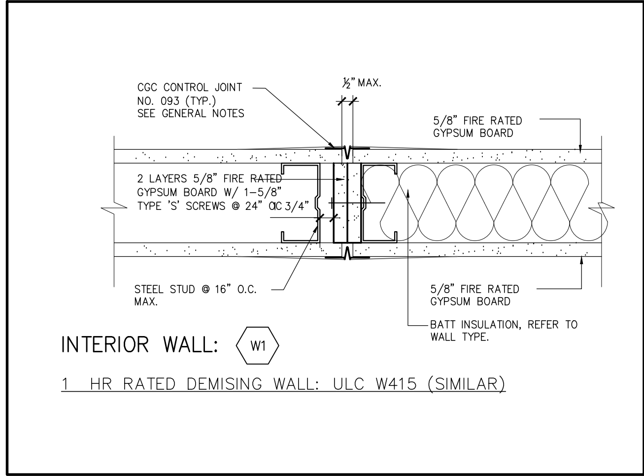
22 PLAN DETAIL SCALE: 3\"/>
