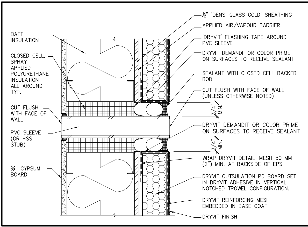
5 SLEEVE THROUGH EIFS DETAIL SCALE: 2\"/>
