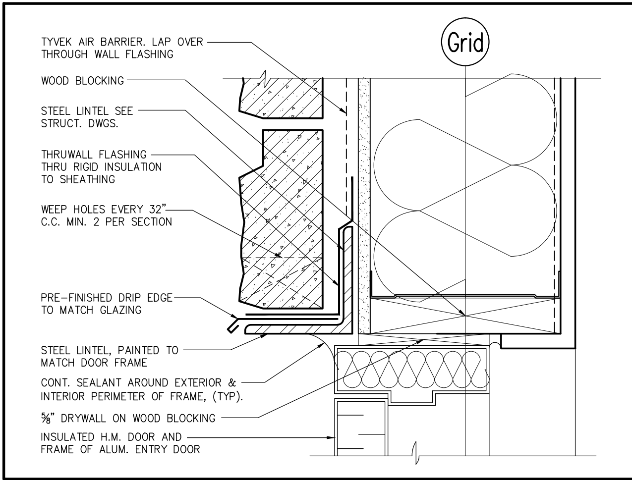
3 SECTION DETAIL SCALE: 3\"/>
