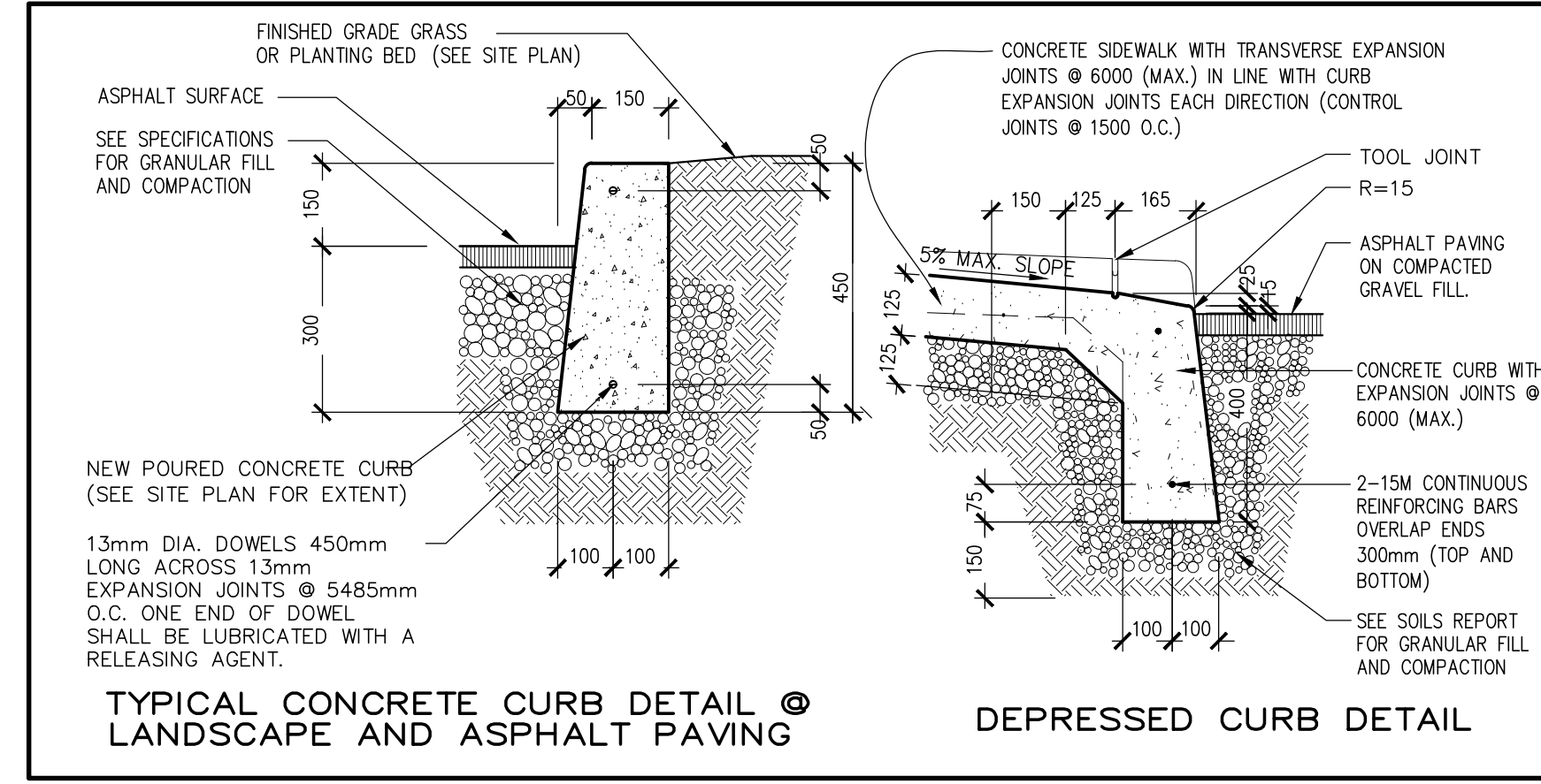
4 TYP. CONCRETE CURB DETAILS SCALE: 1" = 1'-0"
