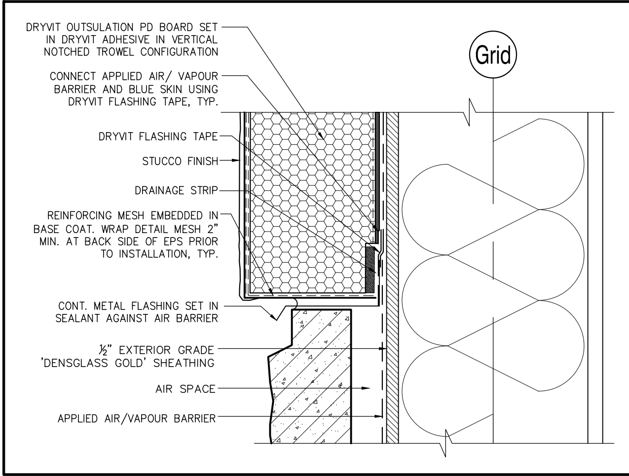
2 SECTION DETAIL SCALE: 3\"/>
