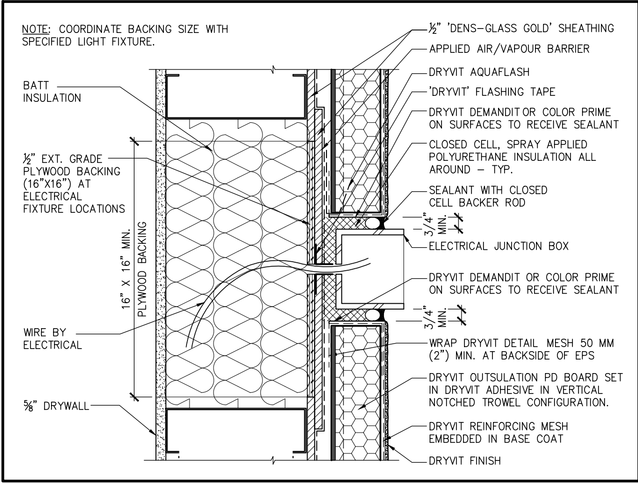
14 SECTION DETAIL SCALE: 2\"/>
