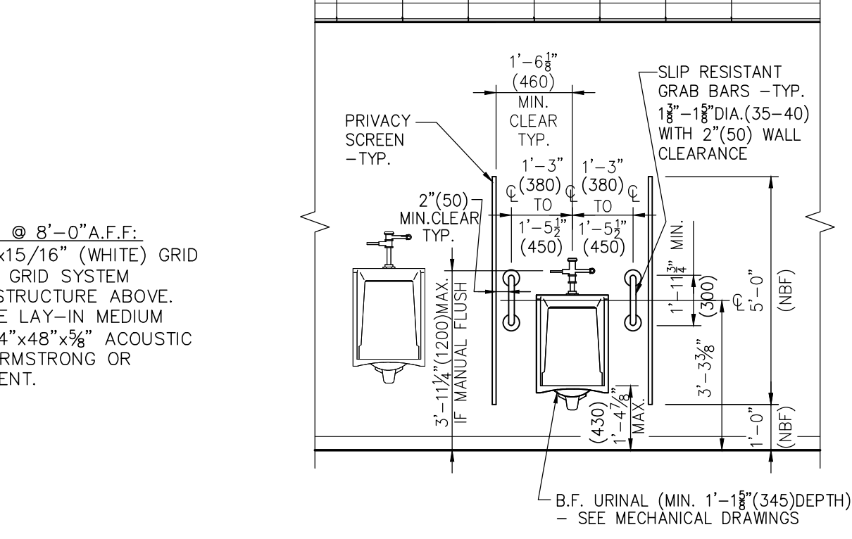
C. ELEVATION (TYPICAL) BARRIER-FREE REQUIREMENTS FOR ONE URINAL WHEN MORE THAN ONE URINAL IS REQUIRED
