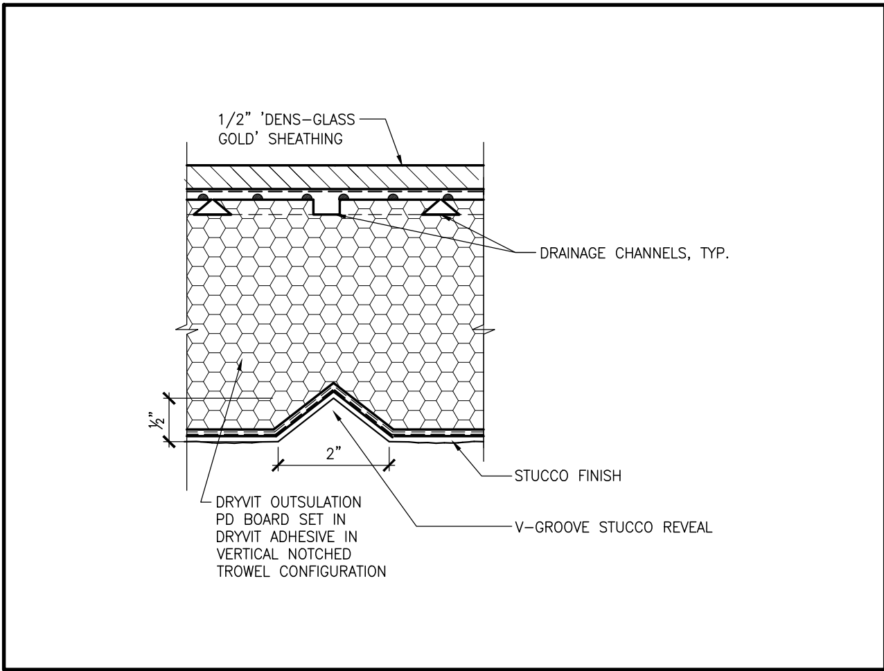
13 TYP. VERTICAL STUCCO REVEAL SCALE: NTS
