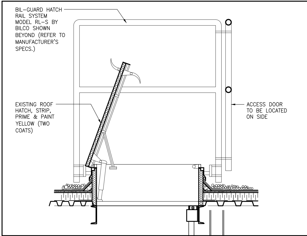
10 ROOF ACCESS GUARD DETAIL SCALE: 3/4" = 1'-0"
