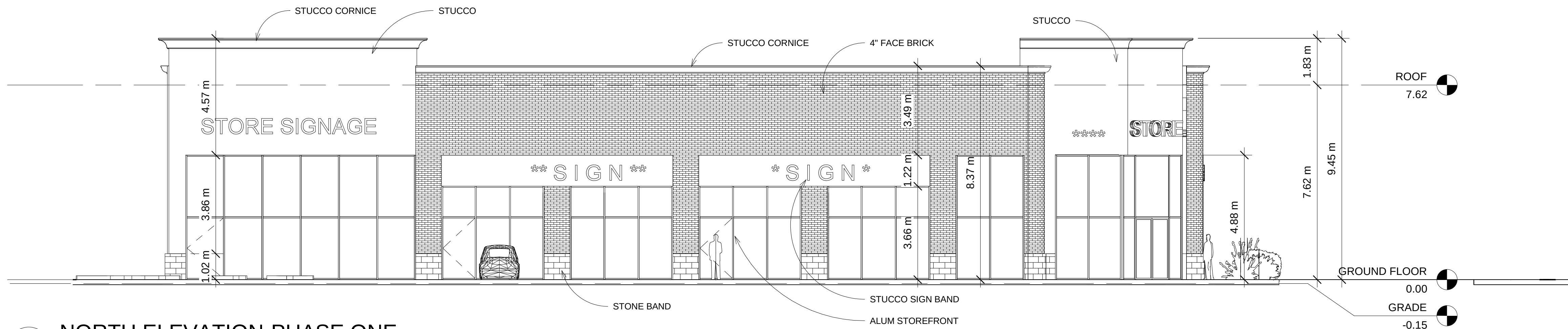
1 NORTH ELEVATION-PHASE ONE 1 : 100
