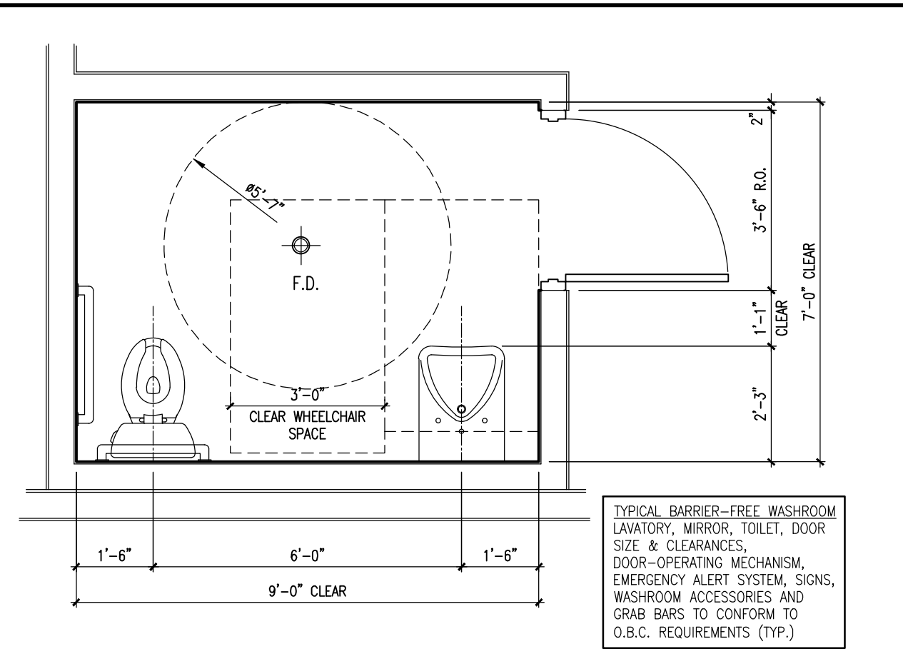
TYP. ENLARGED BARRIER-FREE (UNIVERSAL) WASHROOM LAYOUT
