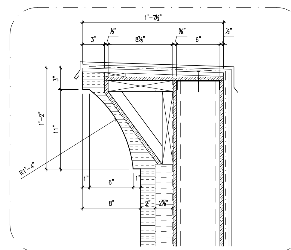
C ENLARGED DETAIL A-5.0 SCALE: 1 1/2" = 1'-0"
