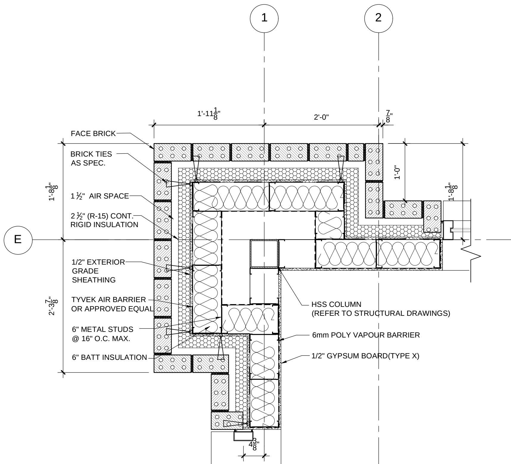
1 A-2.0 PLAN NORTH ENLARGED PLAN SCALE: 1"=1'-0"
