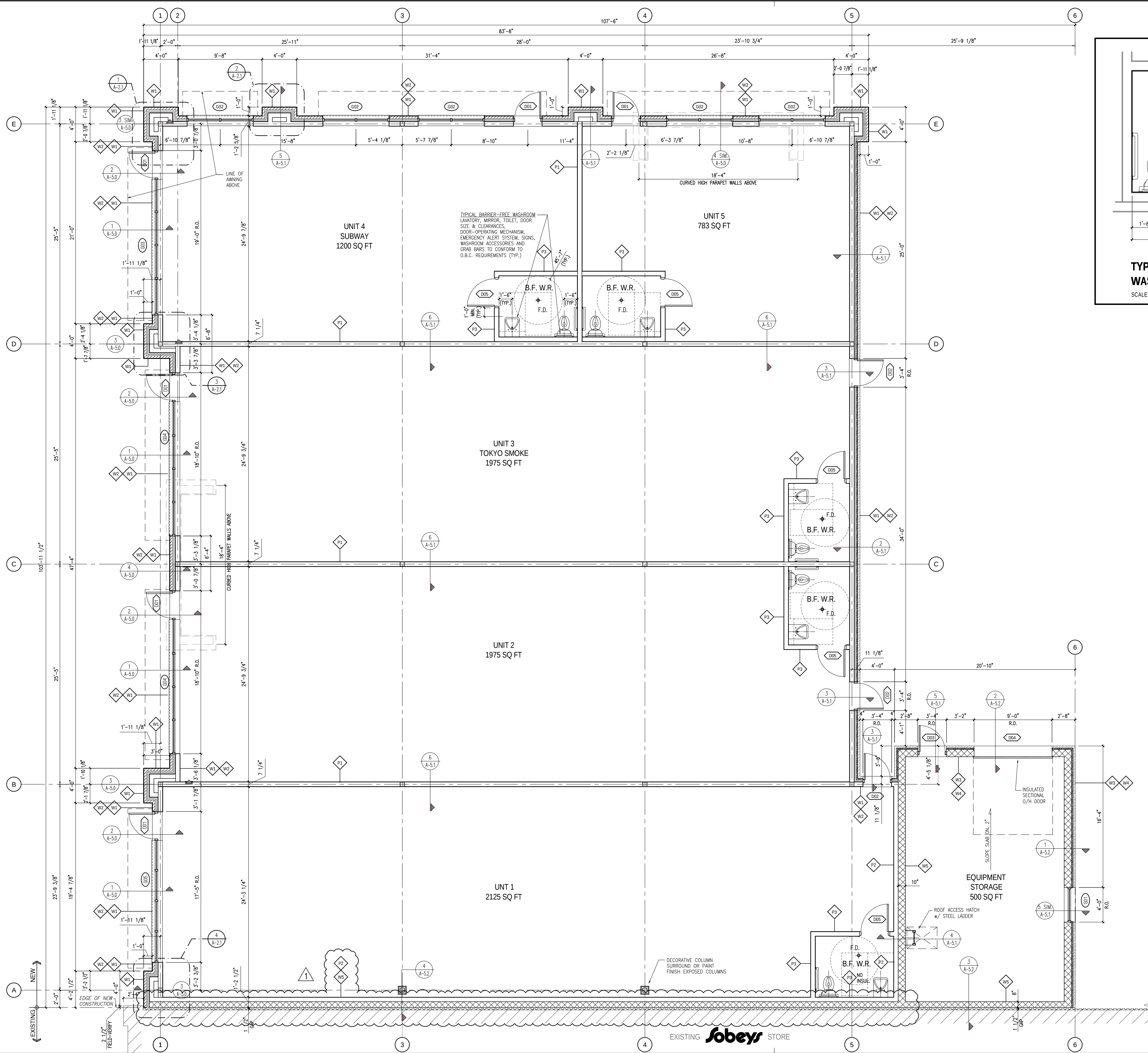
GROUND FLOOR PLAN SCALE: 3/16" = 1'-0"
