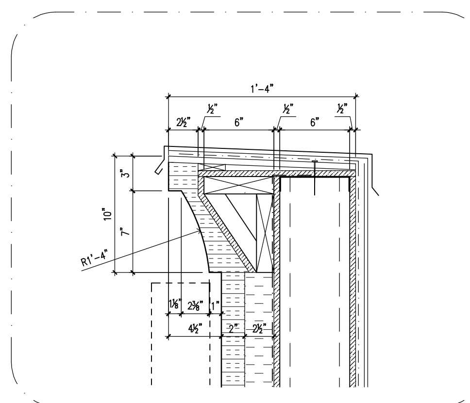
A ENLARGED DETAIL A-5.0 SCALE: 1 1/2" = 1'-0"
