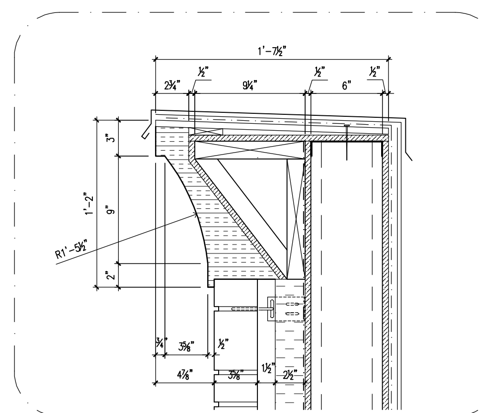
B ENLARGED DETAIL A-5.0, A-5.1 SCALE: 1 1/2" = 1'-0"
