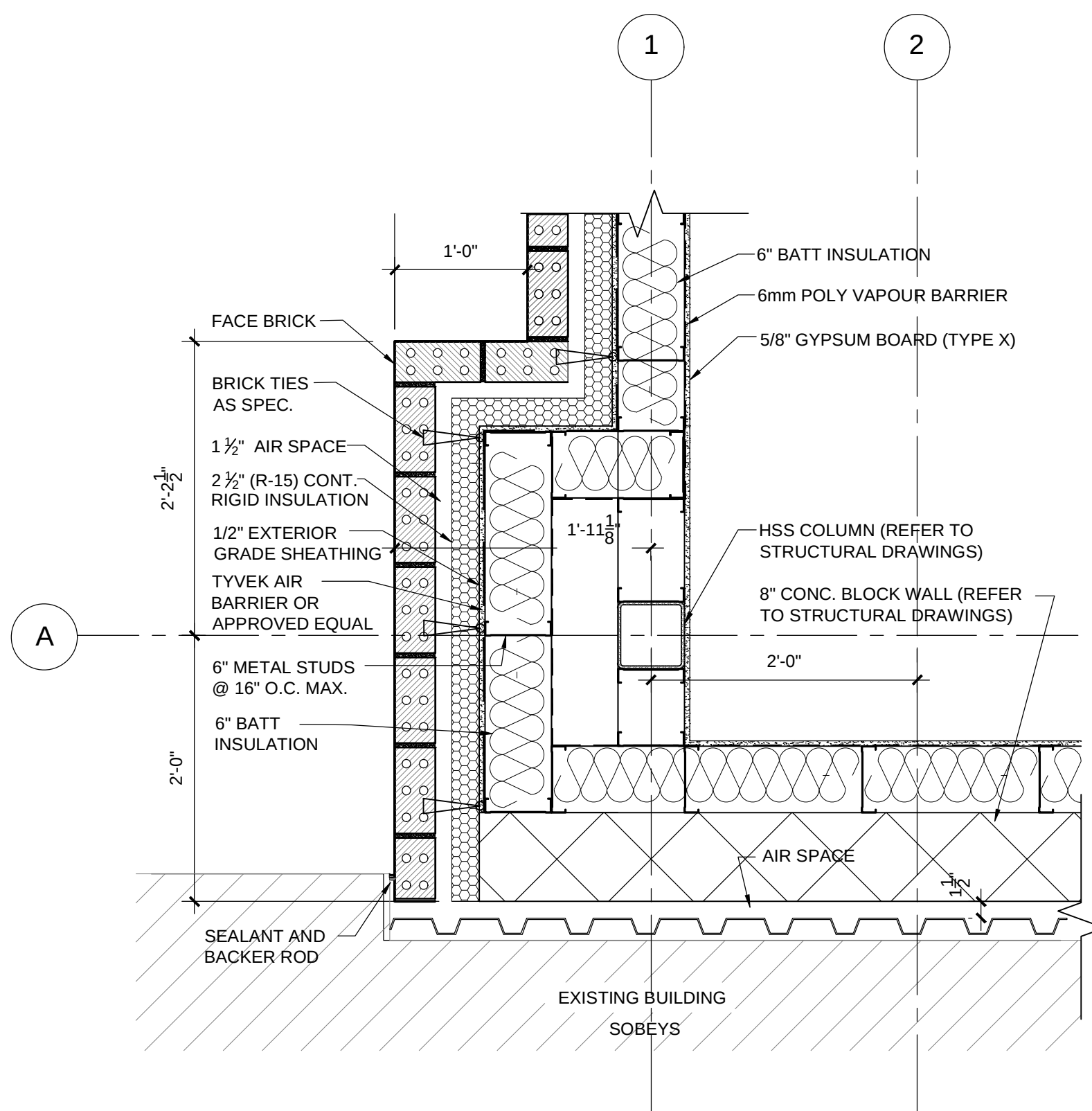
4 A-2.0 PLAN NORTH ENLARGED PLAN SCALE: 1"=1'-0"
