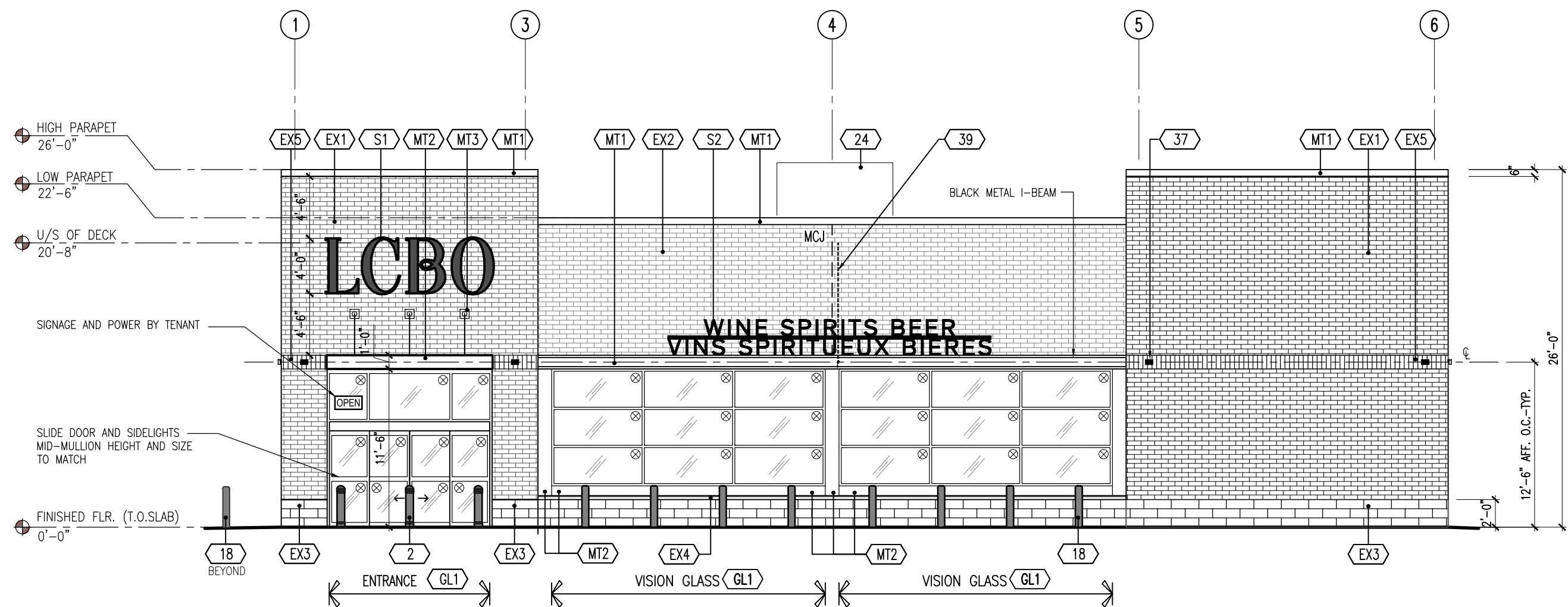
1 EAST ELEVATION (MAIN ENTRANCE) SCALE: 1/8" = 1'-0"
