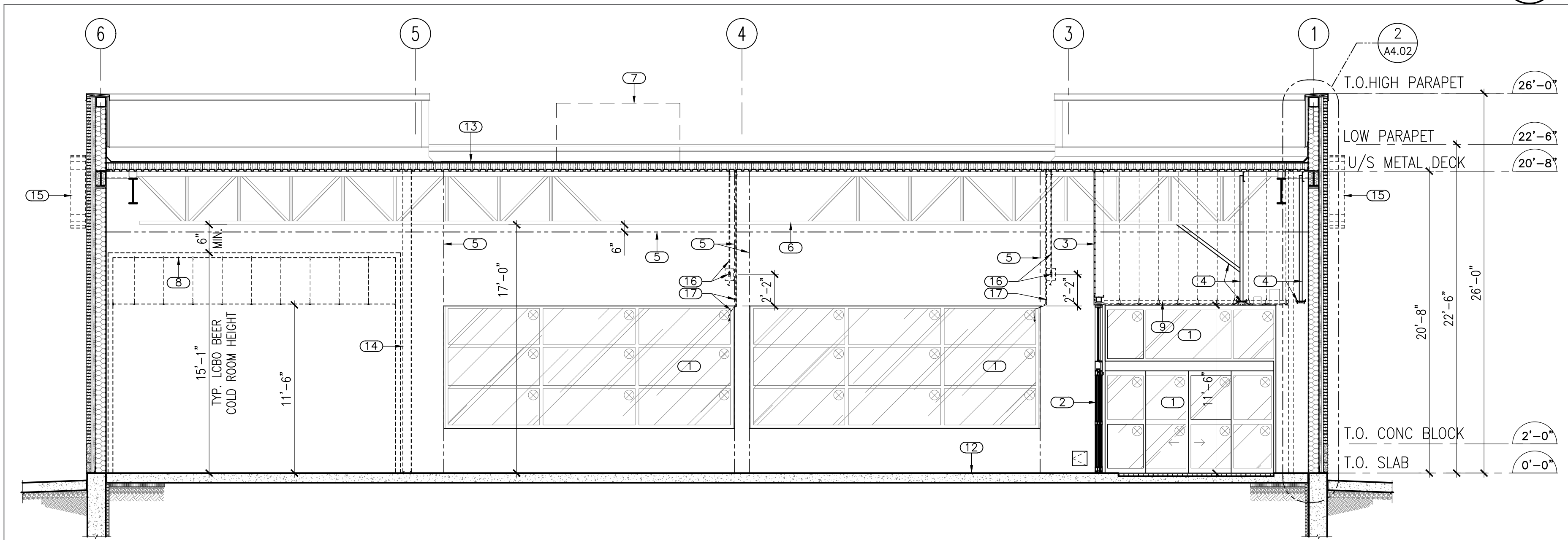
Building Section 1 Scale: 1/8"=1'-0" A4.01
