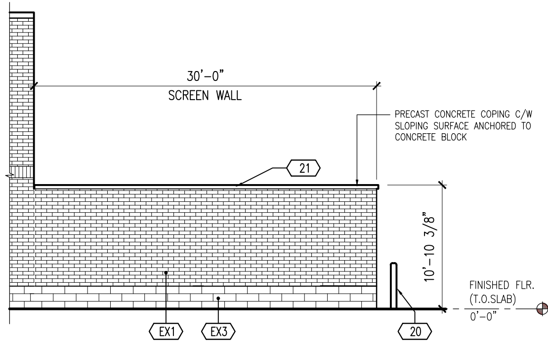
WEST ELEVATION OF SCREEN WALL SCALE: 1/8" = 1'-0"
