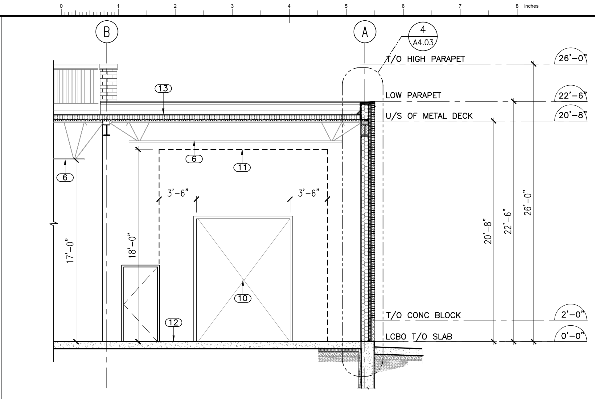
Building Section 3 Scale: 3/16"=1'-0" A4.01
