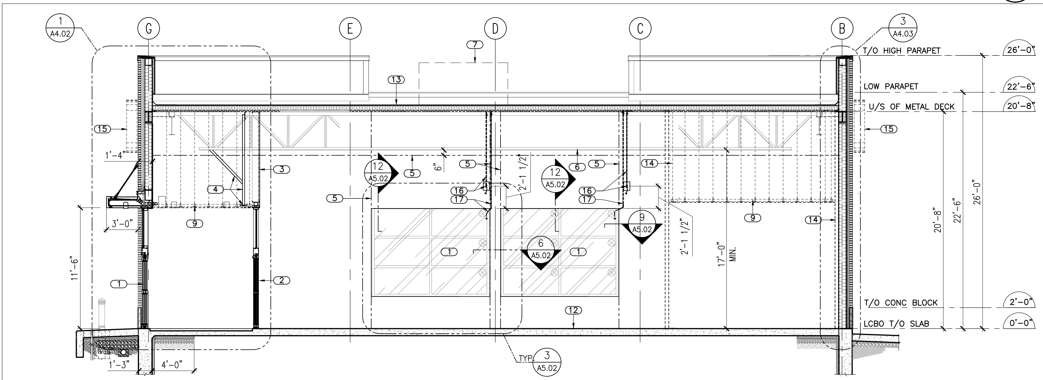
Building Section 2 Scale: 3/16"=1'-0" A4.01
