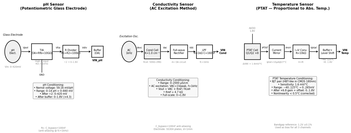
AquaMonitorSoC v1.0 — Sensor Conditioning Circuits Signal conditioning for pH, Conductivity and Temperature channels
