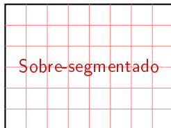
Watershed Tradicional
