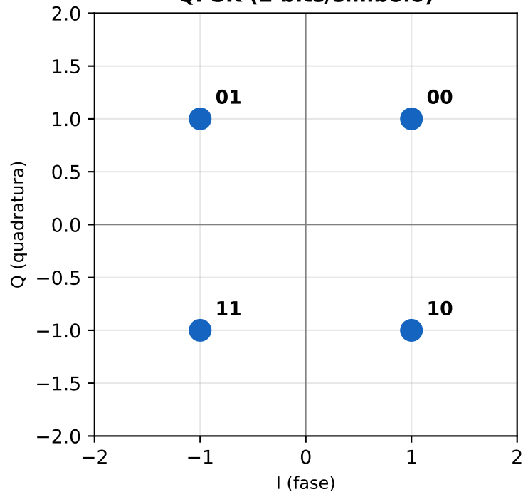
QPSK (2 bits/simbolo)
