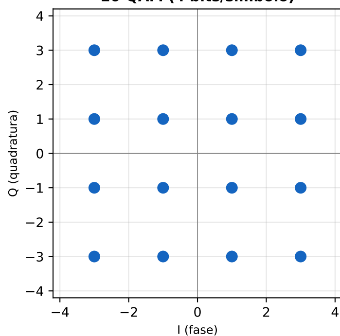
16-QAM (4 bits/simbolo)
