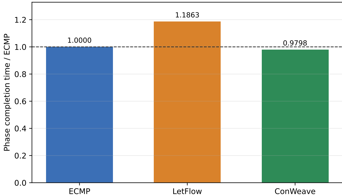
128-host synchronized all-to-all, 4 MiB per flow
