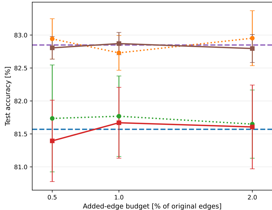
PubMed
