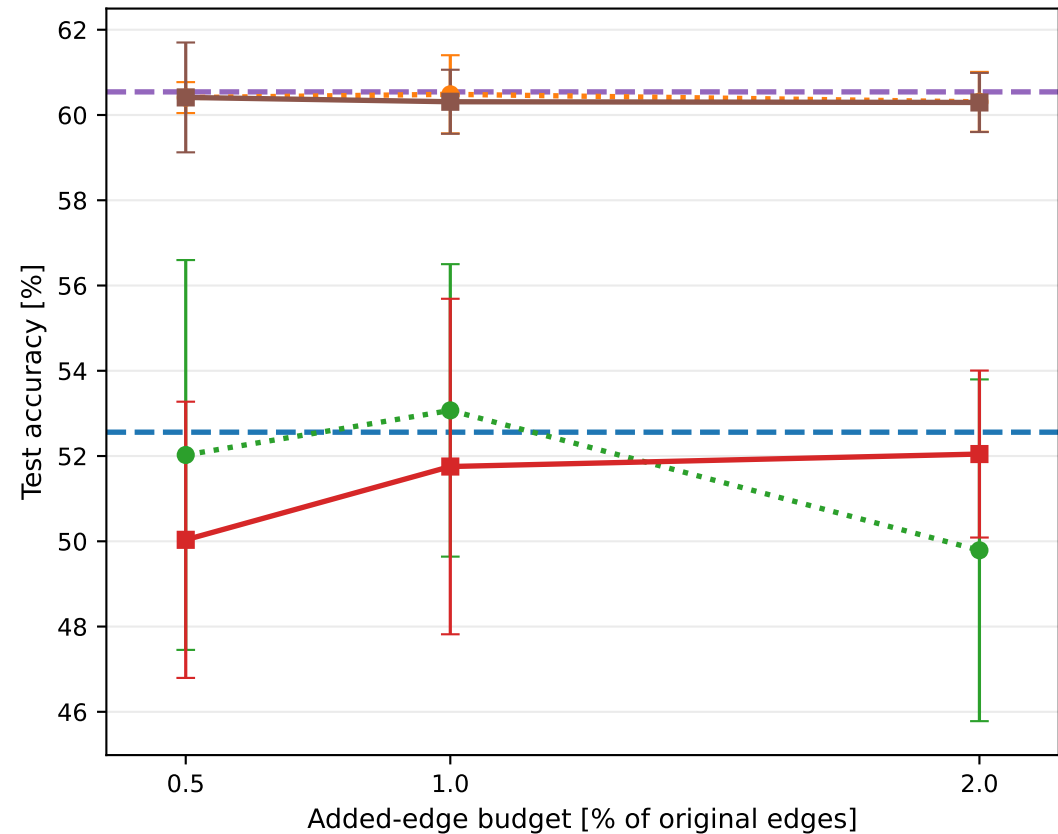
Roman-Empire
