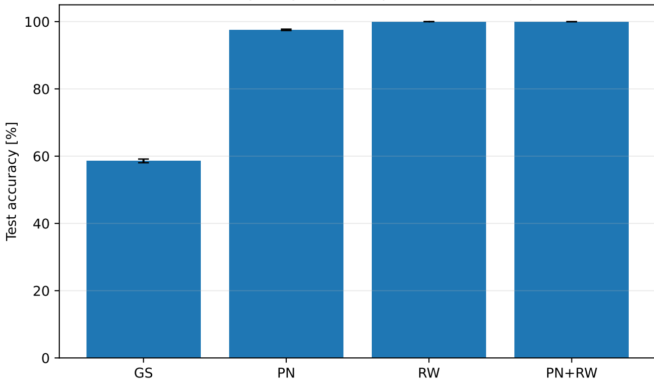
Hard long-range regime: predictive recovery
