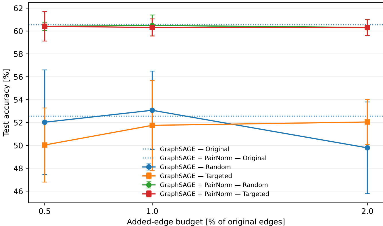
Roman-Empire: accuracy across rewiring budgets
