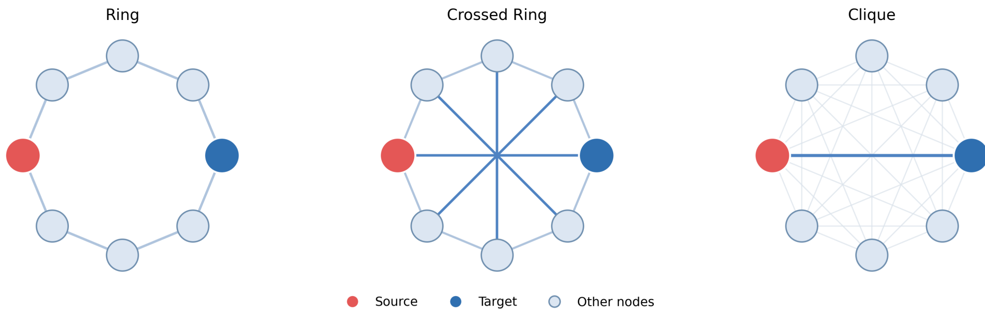
Figure 6: Schematic graph structures illustrating how connectivity can alter long-range information pathways between the same source and target nodes. The ring provides sparse multi-hop routes, the thesis-specific crossed-ring construction augments the ring with opposite-node shortcuts, and the clique provides dense connectivity. This is a conceptual figure, not an empirical result.
