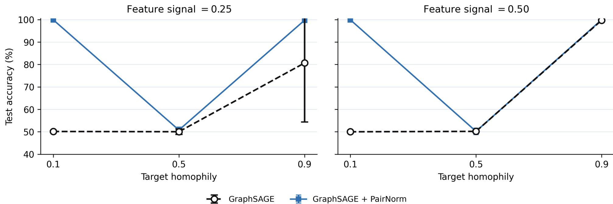
Figure 12: Test accuracy of eight-layer GraphSAGE with and without PairNorm on controlled cSBM graphs across target homophily levels and two feature-signal strengths. Points show means across five coupled graph/training seeds; error bars indicate standard deviations.
