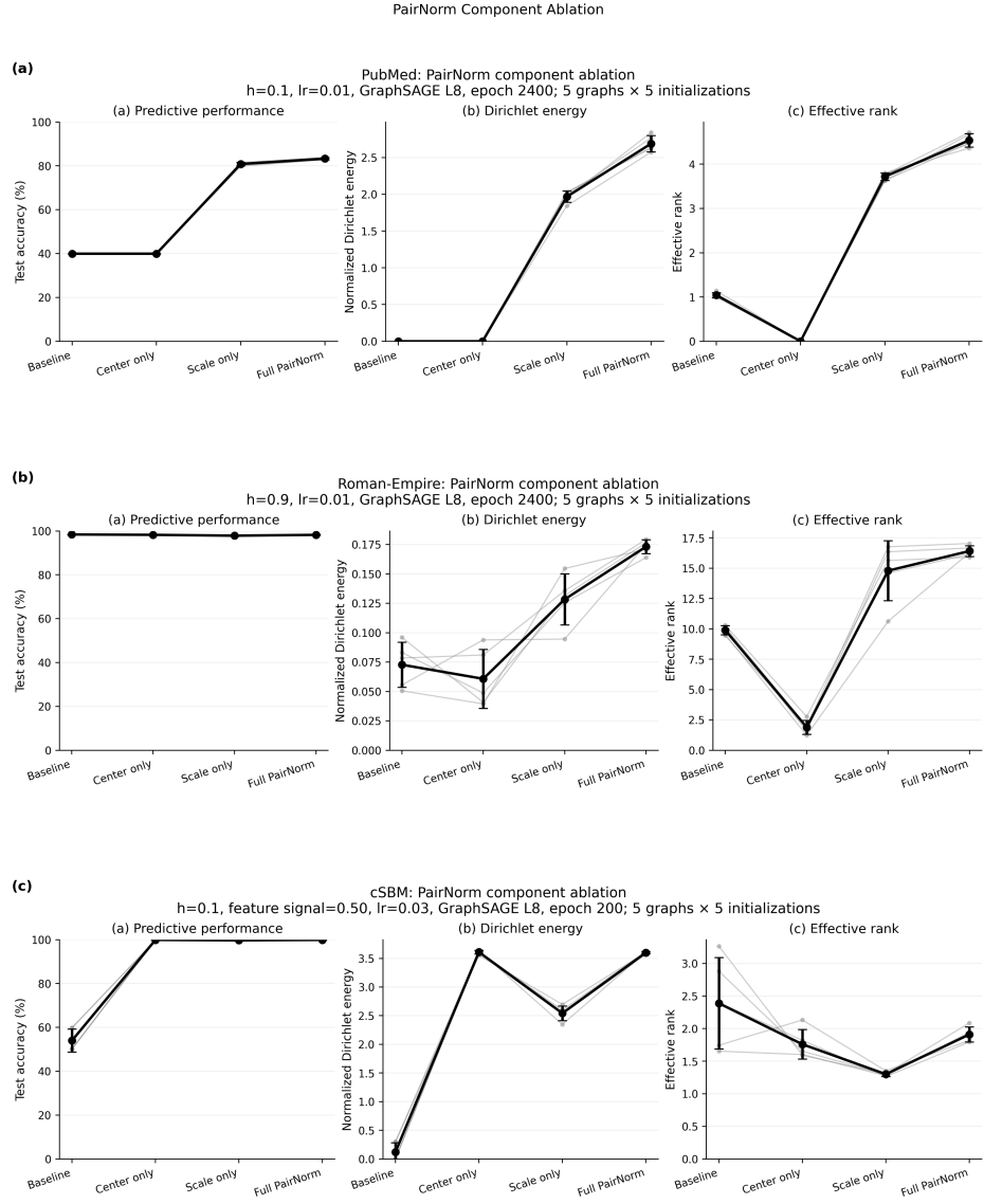
Figure 14: PairNorm component ablations for controlled PubMed, Roman-Empire, and cSBM conditions. Results are first averaged across five model initializations within each graph seed; black markers and error bars show the mean and standard deviation across five graph seeds, while gray lines connect the four variants within each graph seed.
