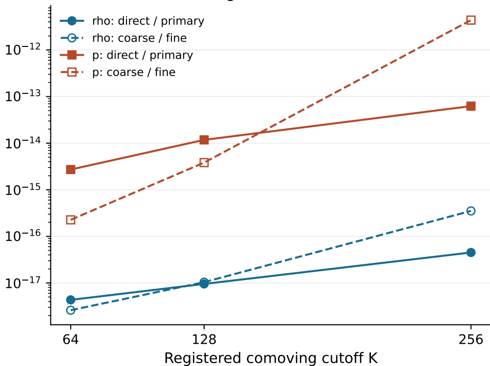
Direct stress agreement and refinement
