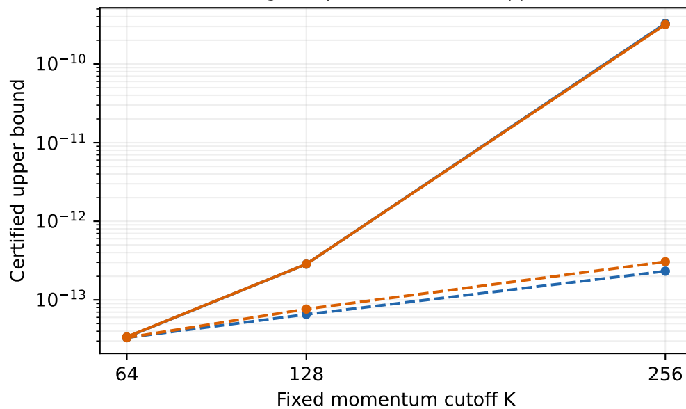
Finite weighted pressure: uniform upper bound
