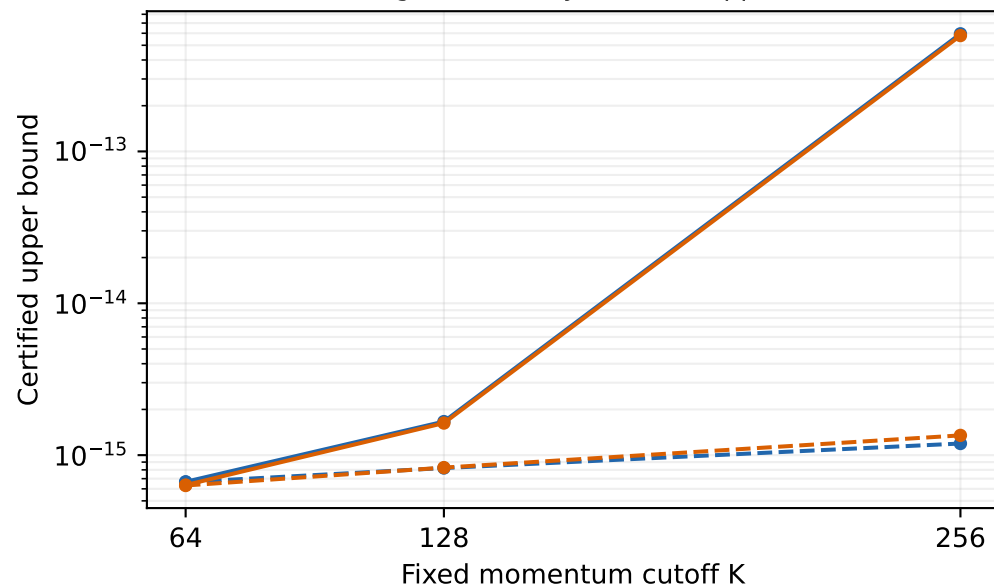
Finite weighted density: uniform upper bound
