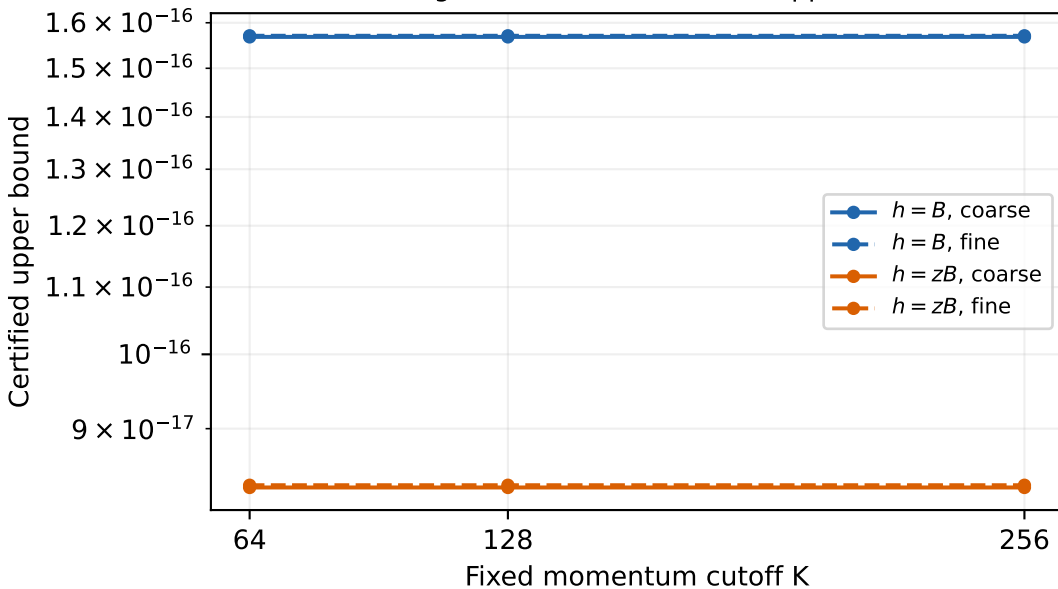
Finite weighted density: uniform upper bound
